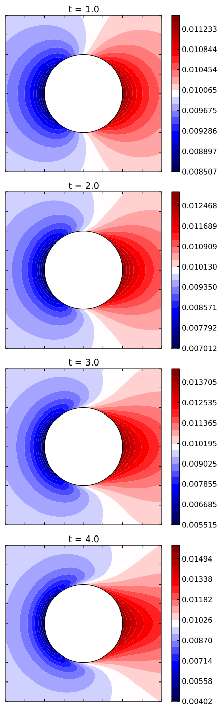
FIGURE 7. Plots showing porosity evolution around a translating sphere. The far field flow is the same as in figures 2 and 3. The sphere has radius a = 0.001 in dimensionless units. Four different times are shown, where time is scaled by a/|\mathbf{V}| . The background porosity is 0.01 and is shown as white on the plots. Red indicates increased porosity from the background, blue shows reduced porosity. Note that a different colourscale is used in each time plot. R = 1000 .
