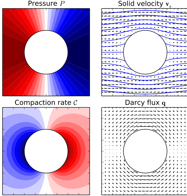
FIGURE 2. Pressure P , solid velocity \mathbf{v}_s , compaction rate \mathcal{C} , and Darcy flux \mathbf{q} for uniform flow past a sphere. The sphere has radius a = 0.001 in dimensionless units (i.e. the compaction length is large compared to the radius of the sphere). The bulk viscosity to shear viscosity ratio R = 1.0 . These plots are similar to those in figure 1 of McKenzie & Holness (2000). Contours in the left hand plot are equally spaced with red indicating positive, blue indicating negative, and white zero. Matrix particle paths are shown as blue lines in the solid velocity plot. Arrows in the right hand plots show the direction and magnitude of the given velocity.
