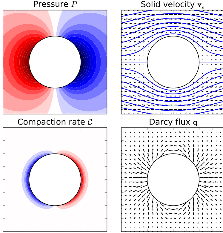
FIGURE 3. Uniform flow past a sphere as in figure 2, except now the sphere has radius a = 10.0 in dimensionless units (i.e. the compaction length is small compared to the radius of the sphere). Compaction is confined to a small boundary layer around the sphere.
