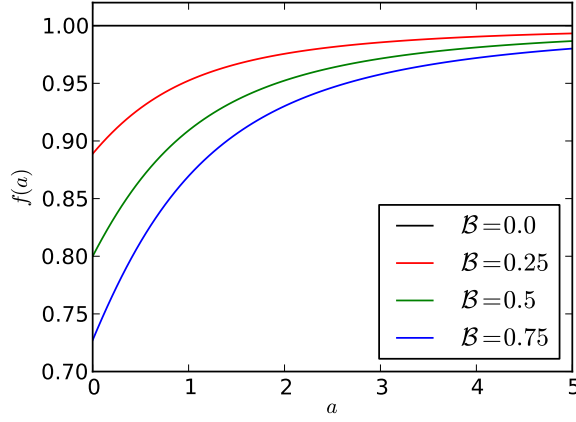
FIGURE 4. Plot of the drag reduction factor f(a) as given in (5.25).
