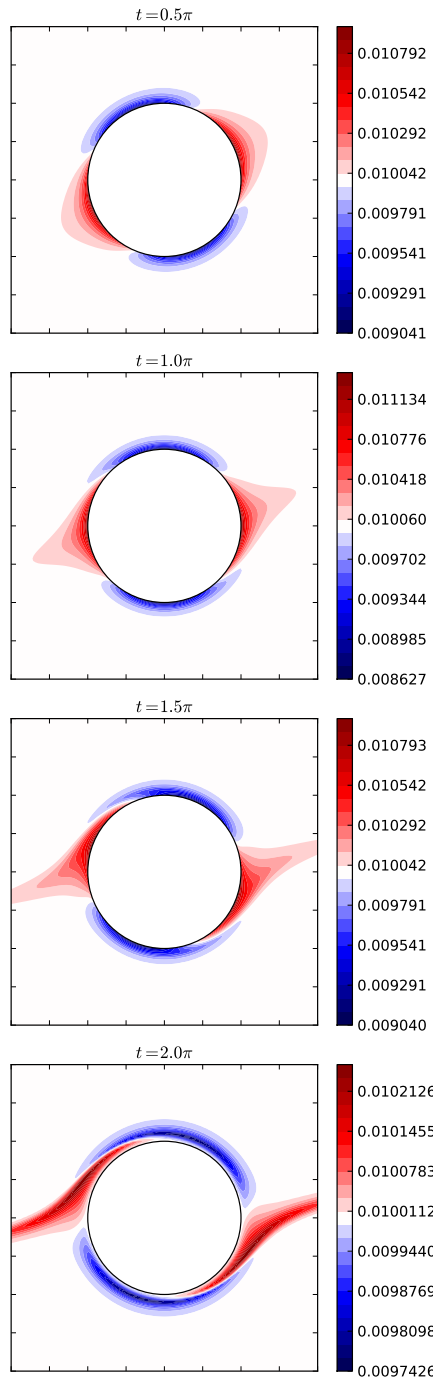
FIGURE 10. Plots showing the porosity evolution around a freely rotating sphere in a simple shear flow as in figure 9 except now the sphere has a dimensionless radius of 10.0. The background porosity and R are unchanged from figure 9.
