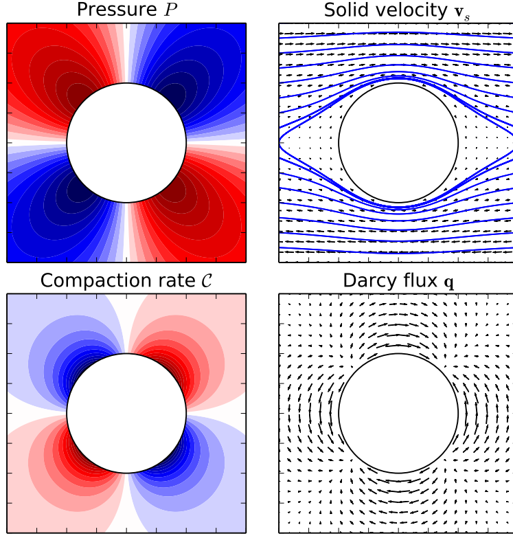
FIGURE 5. Freely rotating sphere in a simple shear flow, with fields as in figures 2 and 3. The sphere has radius a = 0.001 and R = 1.0 . The far field simple shear takes the form \mathbf{v}_s \sim (\gamma y, 0, 0) . Shown are plots of the x - y plane.
