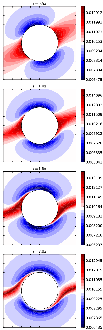
FIGURE 9. Plots showing the porosity evolution around a freely rotating sphere in a simple shear flow. The far field flow is the same as in figures 5 and 6. The sphere has radius a = 0.001 in dimensionless units. Four different times are shown, going up to a total strain of 2\pi , corresponding to a rotation of the sphere by \pi radians. The background porosity is 0.01 and is shown as white on the plots. Red indicates increased porosity from the background, blue shows reduced porosity. Note that a different colourscale is used in each time plot. R = 1000 .
