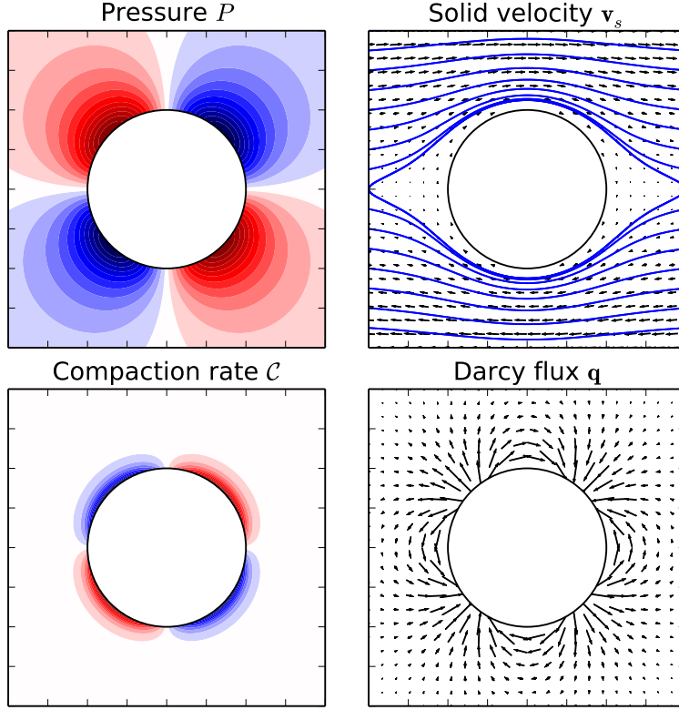
FIGURE 6. Freely rotating sphere in a simple shear flow as in figure 5, except now the sphere has radius a = 10.0 . As before, R = 1.0 .
