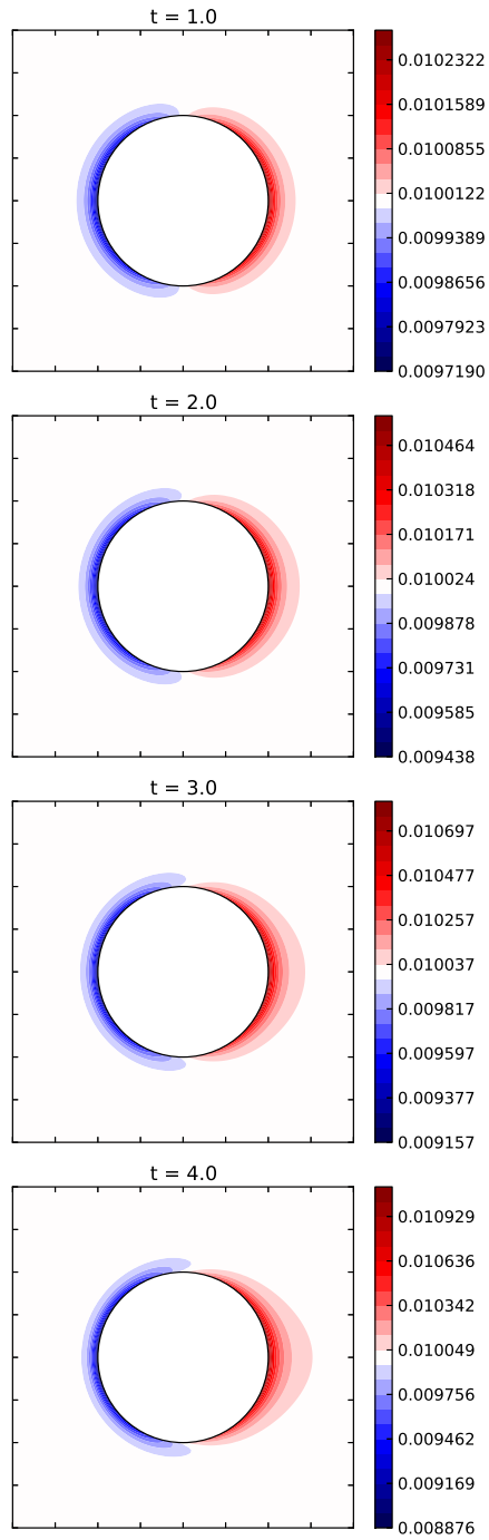
FIGURE 8. Plots showing porosity evolution around a translating sphere as in figure 7 except now the sphere has a dimensionless radius of 10.0. The background porosity and R are unchanged from figure 7.
