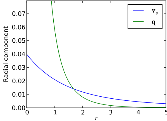
FIGURE 1. Plot of the radial components of v_s and q for a point injection of melt of strength Q = 1 , as given by (4.15) and (4.16).
