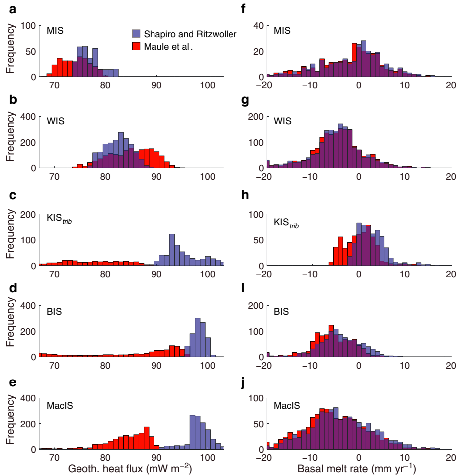
Figure 2. (a–e) Frequency distribution of geothermal heat flux for MIS, WIS, KIS trib , BIS, and MaclS. Blue bars represent data from Shapiro and Ritzwoller [2004], and red bars show data from Maule et al. [2005]. (f–j) Modeled basal melt rates when geothermal heat flux is from Shapiro and Ritzwoller (blue bars) and Maule et al. (red bars).
