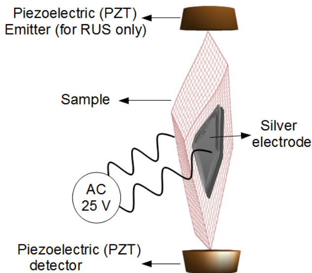
FIG. 1. Schematic diagram of the experimental arrangement for resonant piezoelectric spectroscopy (RPS). The same setup can be used for resonant ultrasonic spectroscopy (RUS) by applying the ac voltage across the top piezoelectric transducer rather than the electrodes coating two parallel surfaces of the sample. The applied ac voltage for RPS and RUS measurements on \text{SrTiO}_3 was 25 V.
