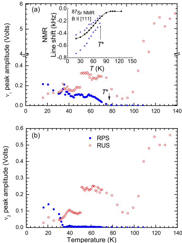
FIG. 4. The temperature evolution of the amplitudes of the mechanical resonances \nu_1 and \nu_2 observed using RPS and RUS measurements on \text{SrTiO}_3 . (a) RPS (filled blue circles) and RUS (red empty circles) amplitudes of \nu_1 . The inset in part (a) shows the temperature dependence of the central 1/2 \leftrightarrow -1/2 ^{87}\text{Sr} NMR transition at 9.2 T for \mathbf{B} \parallel [111] in \text{SrTiO}_3 which is split into three components at T < T^* \approx 75 - 80 K. The black squares represent the central NMR component that exhibits tetragonal symmetry whereas the triangles are the frequencies of satellite peaks, which exhibit non-tetragonal symmetry. (b) RPS (filled blue circles) and RUS (red empty circles) amplitudes of \nu_2 . The uncertainty in RPS and RUS amplitudes is estimated to be 10%, which mainly stems from the mechanical coupling between the sample and transducers which may change by thermal contraction.
