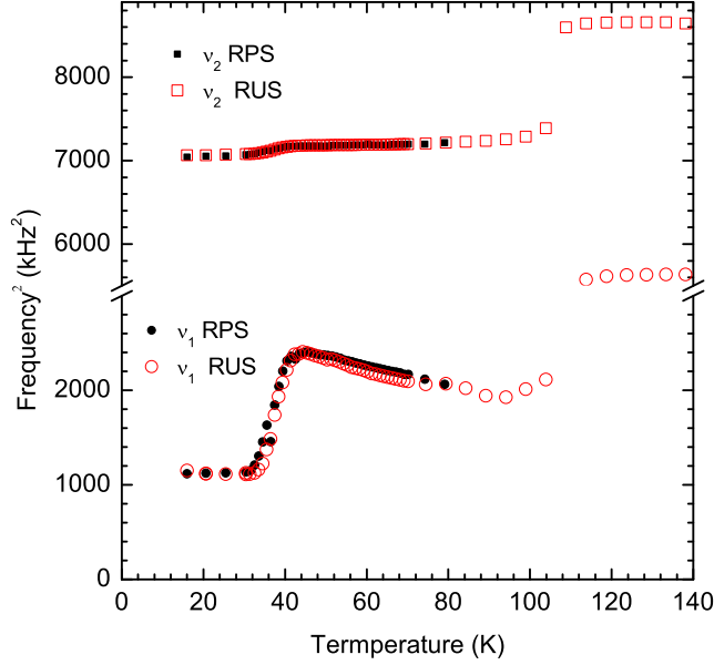
FIG. 3. The temperature evolution of the frequency of the mechanical resonance \nu_1 (black, filled circles and empty, red circles) and \nu_2 (black, filled squares and empty, red squares) determined using RPS and RUS. The agreement of results from RPS and RUS confirms that Fano-like features observed in the RPS spectra correspond to mechanical resonances of \text{SrTiO}_3 , giving direct evidence of polarity in \text{SrTiO}_3 .
