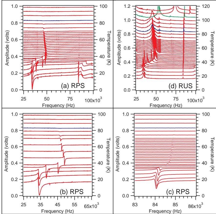
FIG. 2. Low temperature RPS and RUS spectra of SrTiO 3 . Panel (a) Segments of RPS spectra in the frequency interval from 25 kHz to 100 kHz. The spectrum shown in blue was collected at T^* \approx 80 K. Disappearance of two mechanical resonances located at \nu_1 \approx 40 kHz and \nu_2 \approx 85 kHz with increasing temperature is shown in panels (b) and (c). Panel (d) shows segments of RUS spectra in the same frequency interval as in panel (a) for comparison. The spectrum shown in green was collected at the cubic-tetragonal ferroelastic transition temperature T_c = 105 K. In all panels the left axis represents the amplitude and the right axis gives the temperature at which each spectrum was collected.
