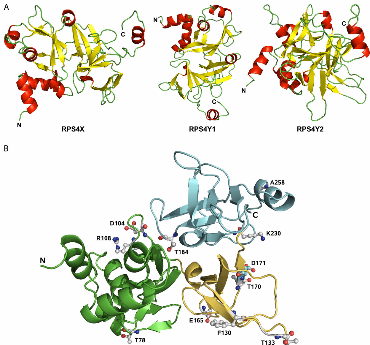
Figure 4 Three dimensional models of isolated RPS4 proteins. The N and C termini are marked. (A) Structure of each RPS4 protein. \beta strands are in yellow, \alpha helices in red and loops in green. (B) RPS4X showing the one residue that is different in the three RPS4 proteins (carbon atoms in cyan, oxygen atoms in red and nitrogen atoms in blue) and the residues that are different, with non-conservative substitutions, in one or both of the RPS4Y proteins (carbon atoms in grey, oxygen atoms in red and nitrogen atoms in blue). N-terminal domain is in green, central domain in yellow and C-terminal domain in cyan.
