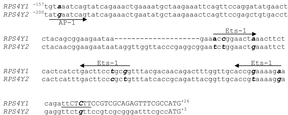
Figure 3 Sequence motifs found within the promoter regions of RPS4Y1 and RPS4Y2 . The numbers indicate nucleotide positions relative to the TSS, according to [18]. For RPS4Y2 , we considered that the TSS overlaps the ATG. Hyphens represent inserted/deleted nucleotides. The oligopyrimidine tract overlapping the RPS4Y1 transcription start site is underlined. Arrows indicate the orientation of the predicted transcription factor binding sites (forward or reverse strand). The positions within the sequence motifs that differ between the two genes are in italic.
