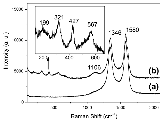
Fig. 2 Raman spectrum of CNTs before (a) and after (b) ALD of ZnO. Inset : Raman spectrum in the range of 150–650 \text{cm}^{-1} of ZnO-coated CNTs
