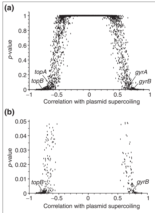
Figure 1 Significance versus correlation of gene expression and plasmid supercoiling values for all genes over all experiments. For each gene we computed the correlation coefficient between its gene expression ratios (base 2 logarithm) over all experiments with the superhelical density ( \sigma ) of a reporter plasmid, as measured by gel electrophoresis. These values are plotted against the p -value, which represents the chance that the difference in expression between relaxation and control experiments could have arisen randomly. (a) Scatter plot for all genes. There is a general trend in which genes with low p -values showed very high correlation (absolute value) between expression and plasmid supercoiling. The points corresponding to the topoisomerase genes gyrA , gyrB , topA and topB are indicated. (b) Expanded portion of (a) highlighting those genes classified as significant ( p < 0.05 ). Genes with very low p -values show high positive or negative correlation between expression and plasmid supercoiling.
