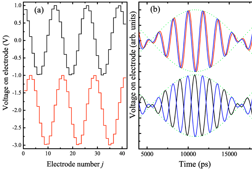
FIG. 2. (a) The upper curve shows the instantaneous values of the voltages on the 41 upper electrodes of the array; \eta/2\pi=552.653 MHz and \Delta t = 140 ps, corresponding to v \approx 1.063c for a\Delta\varphi=44.6 mm [see Eq. (3)]. The resulting polarizations under the electrodes will be proportional to these voltages. The lower curve (offset for clarity) gives the instantaneous voltages 420 ps later; the polarization wave has moved along the dielectric. (Note that the \cos \Omega t term in Eq. (3) hardly changes during this time.) (b) Example of the time-dependent voltages on array electrodes 20 and 21 (upper curves) and 20 and 26 (lower curves) for the same parameters as in (a). Note that the lower-frequency temporal modulation of each electrode voltage produced by the second cosine term in Eq. (3) (dotted curves) is in phase for all electrodes.
