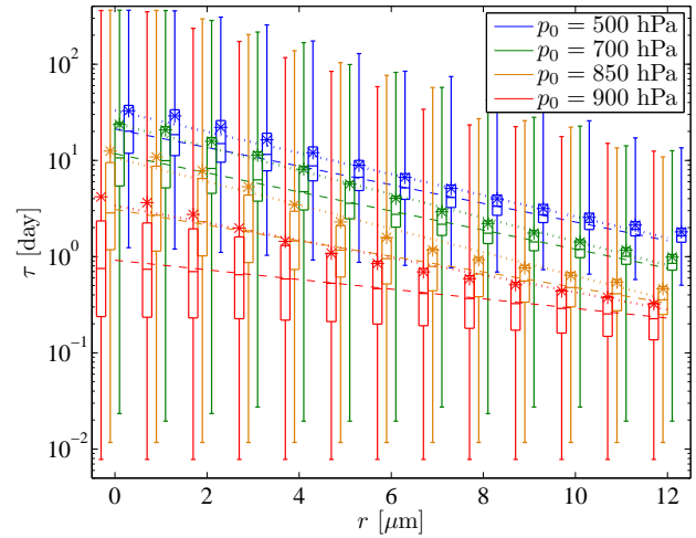
Fig. 4. Statistics of the residence time for different initial levels for n_0 = 2.5 \times 10^5 particles, including the effect of rain and turbulent diffusion (setup 1). Minimums and maximums (lower and upper lines), upper and lower quartiles (boxes), medians (lines in the boxes) and averages (stars) are indicated. Dashed and dotted lines indicate exponential fittings to median and average vs. r for given initial pressure levels.
