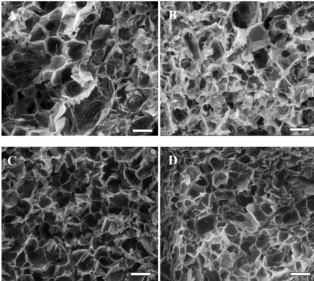
Figure 2-7. SEM images of the (A) 0.03g/ml AA-GMA, (B) 0.05g/ml AA-GMA, (C) 0.06g/ml AA-GMA, (D) 0.07g/ml AA-GMA freeze-dried hydrogen. The bar is 100 \mu m.
