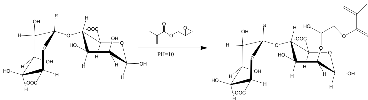
Figure 2-5. Reaction Scheme of the macromonomer AA-GMA
