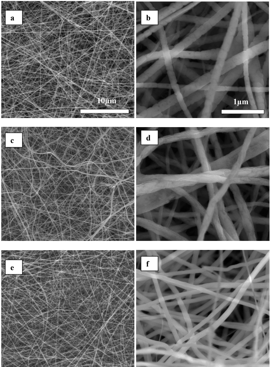
Figure 3-1. SEM images and analysis of the morphology of the electrospun nano-fiber silica-titania meshes produced with (a,b) 6% PVP TiO 2 (c,d) 10% PVP TiO 2 (e,f) silica-titania50/50
