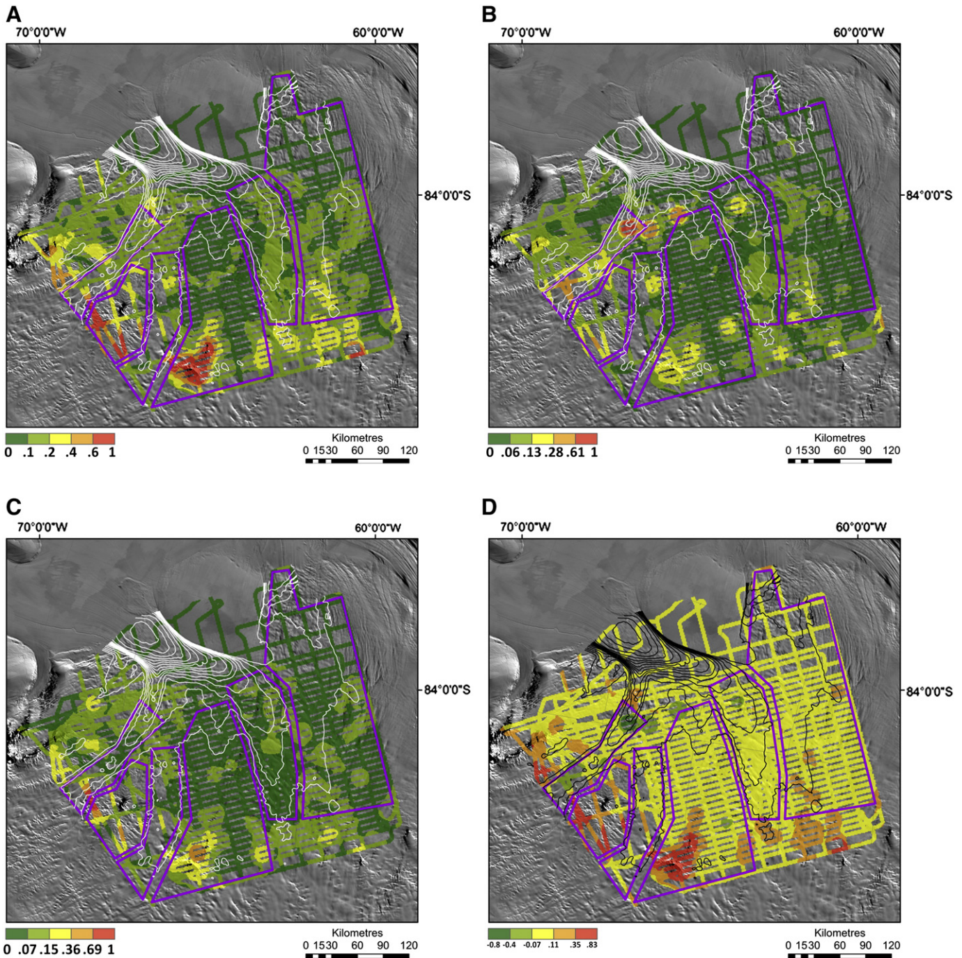
Fig. 4. Normalised (A) total ( \xi_r ); (B) wavelength ( \eta^{-1} ) and (C) slope ( \xi_{sl} ) roughness of the entire IIS/MIS region. In all three images, lower roughness areas are shaded green while higher roughness areas are shaded red. The background image is the MODIS mosaic of Antarctica (Haran et al., 2005; Scambos et al., 2007), and contours of InSAR velocities (after Rignot et al., 2011) are superimposed to indicate the location of the IIS and MIS. Purple boxes delineate our previously defined zones (see Fig. 1A for an indicator of the naming conventions for each area). (D) Plot of \zeta which highlights regions of the bed with distinct roughness characteristics. Although we cannot interpret values of \zeta precisely, clearly the lowest values (the dark green areas), which indicate where \zeta \rightarrow -1 , represent type I regions. Similarly, the moderate values (the yellow areas), which indicate where \zeta \rightarrow 0 , represent type II regions, while the highest values (the red and orange areas), which indicate where \zeta \rightarrow +1 , represent type III regions.
