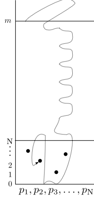
Figure 3: A path from p(m) to INC
