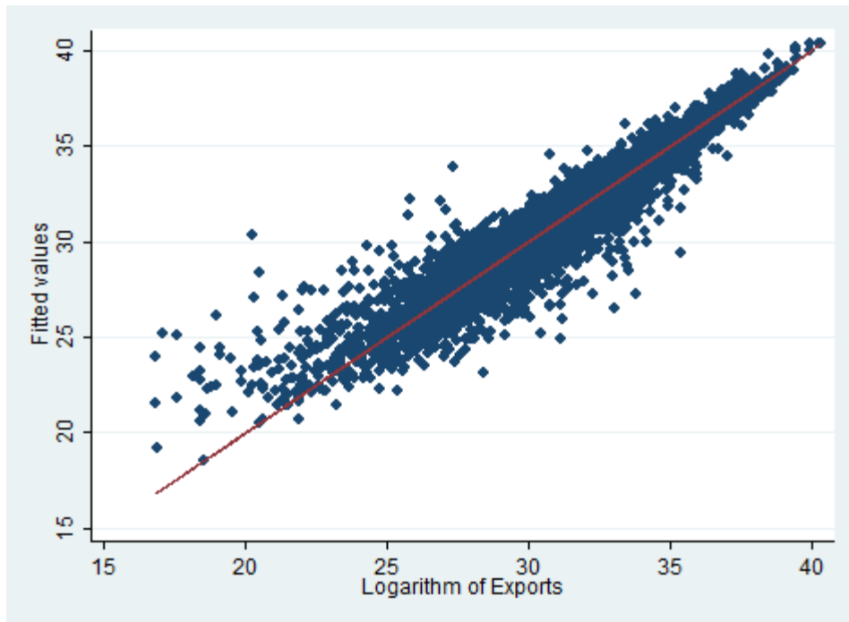
Fig. 6 Heckman model
