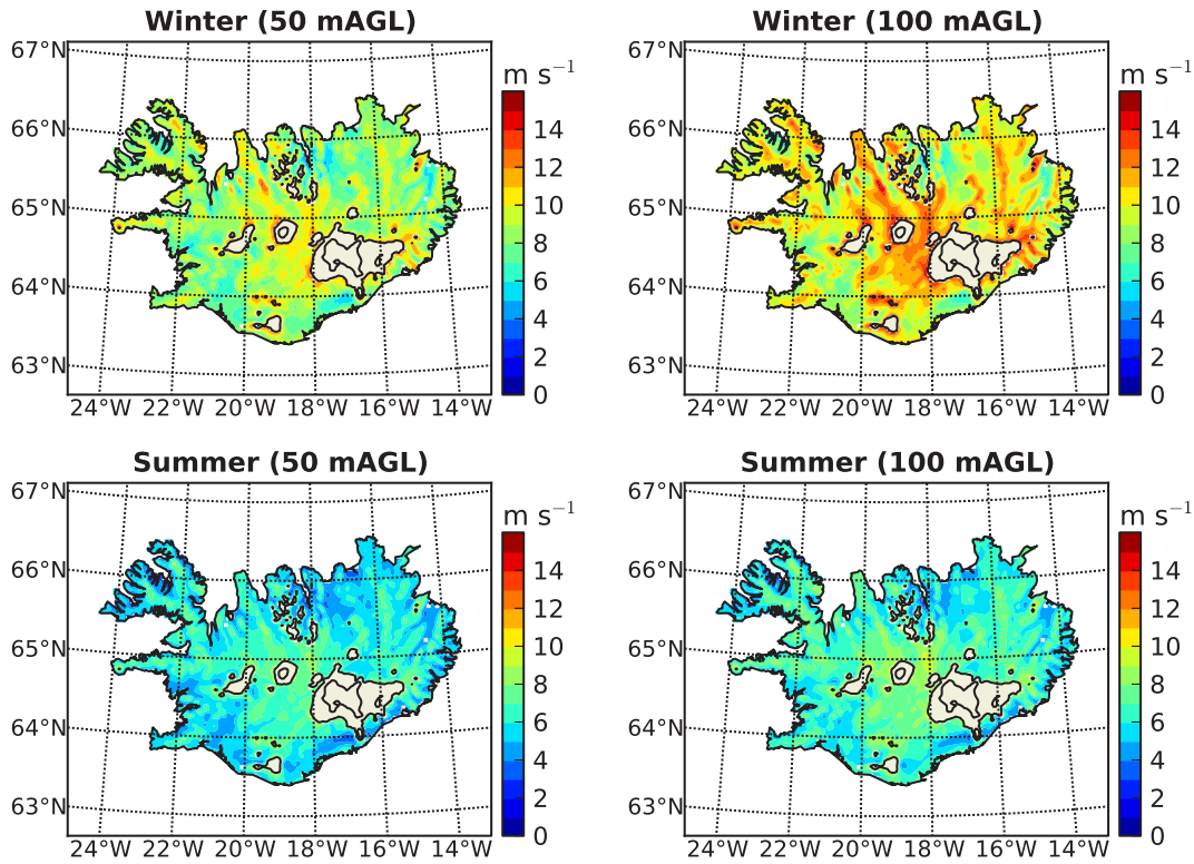
Fig. 5. Winter (DJF) and summer (JJA) averages of wind speed at 50 and 100 m above ground level, based on corrected WRF model data.
