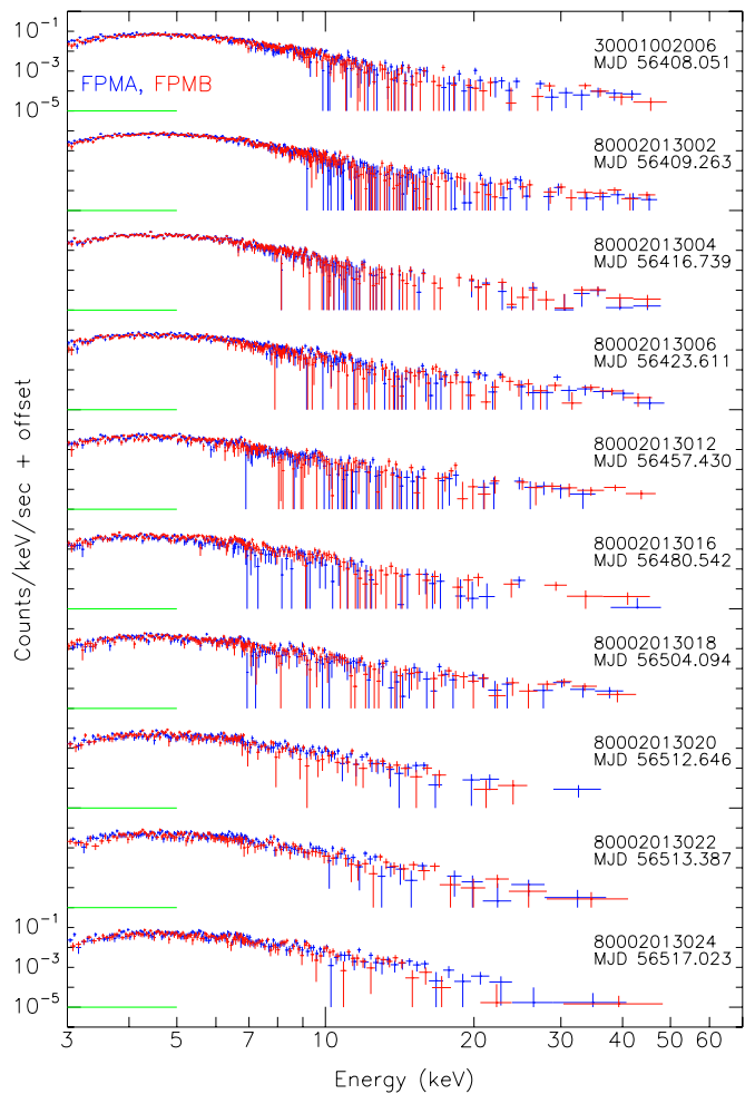
Figure 5. Spectra for all NuSTAR observations from earliest (top) to latest (bottom). FPMA is plotted in blue and FPMB is plotted in red. Spectra have been grouped to have a minimum of 20 counts per spectral bin.
