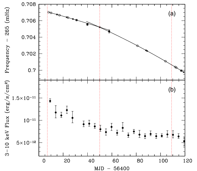
Figure 4. (a) Spin frequency vs. time. The two solid lines represent the two different phase-coherent solutions discussed in Section 2.1 and presented in Table 2. Open circles and stars represent epochs of NuSTAR and WT-mode Swift XRT observations, respectively (see Table 1) with the frequencies calculated from the phase-coherent ephemerides. Note the overlap region between NuSTAR observations on MJDs 56439 and 56457 where both solutions can reasonably fit the phase data; locally calculated frequencies for those data sets are shown in solid circles along with error bars. The dotted vertical red lines indicate epochs of Swift BAT reported bursts on MJDs 56407 (April 25), 56450 (June 7), and 56509 (August 5). (b) Absorbed 3–10 keV flux vs. time in five-day averages from PC-mode Swift XRT observations. The gap in coverage near MJD 56430 was when nearby Transient 1 contaminated the magnetar fluxes (Dufour et al. 2013; Degenaar et al. 2013).
