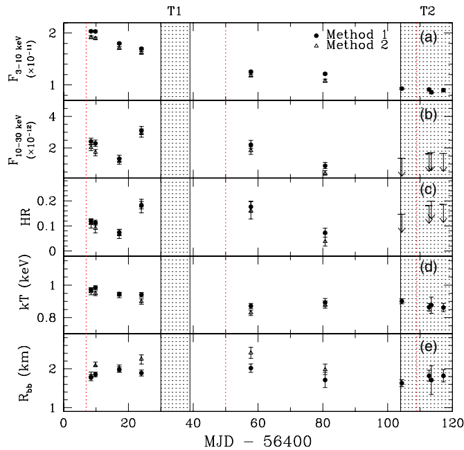
Figure 6. (a) Absorbed flux vs. time in the 3–10 keV band in \text{erg s}^{-1} \text{cm}^{-2} , for Method 1 (solid circles) and Method 2 (open triangles). (b) Absorbed flux vs. time in the 10–30 keV band in \text{erg s}^{-1} \text{cm}^{-2} , for Methods 1 and 2. Note that when Transient 2 is on, we present only upper limits for Method 1 and no values for Method 2. (c) Hardness ratio (defined as the ratio of the 10–30 keV to 3–10 keV absorbed fluxes), showing results from Methods 1 and 2. (d) Blackbody temperature kT for both methods. (e) Blackbody radius R_{\text{bb}} in km for both methods, obtained assuming a distance to the source of 8.0 kpc. All panels: hatched regions indicate epochs when Transient 1 (T1) and Transient 2 (T2) contaminated our NuSTAR data; data for SGR J1745–2900 when T1 was on were unusable for flux or spectroscopy. Vertical dotted red lines indicate epochs of X-ray bursts from the source direction.
