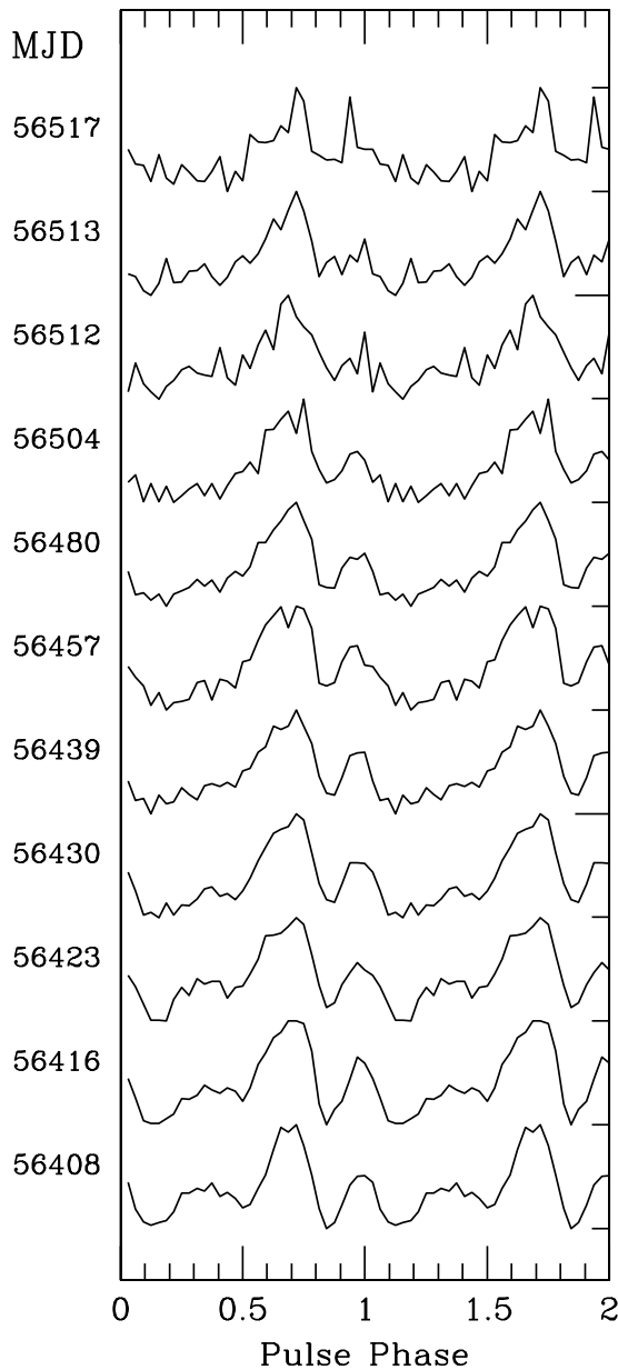
Figure 1. NuSTAR pulse profiles in the 3–10 keV band at the observing MJDs (see Table 1), aligned using the ephemerides presented in Table 2. Two cycles are shown for clarity. Note the gradual disappearance of the first of the three peaks seen in the MJD 56408 observation. Uncertainties on phase bins are omitted for clarity but are well represented by the off-pulse scatter.
