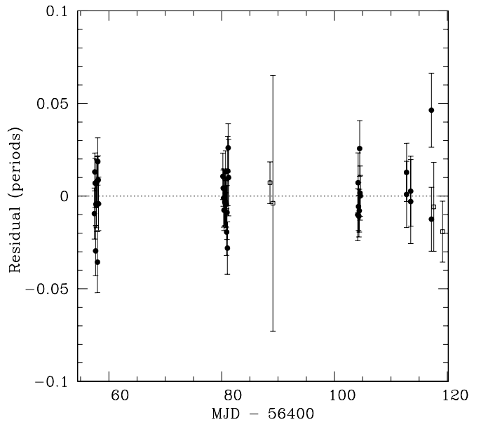
Figure 2. Residuals for the second phase-coherent timing solution shown in Table 2 for the appropriate MJD range. Filled circles are NuSTAR TOAs and empty squares are Swift TOAs.
