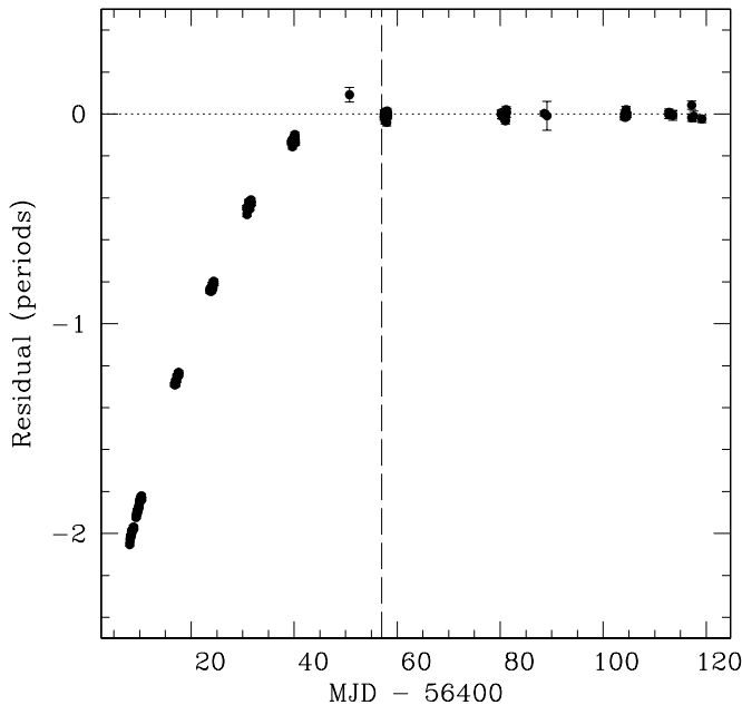
Figure 3. Attempt to extrapolate the second timing solution backward, showing growing phase deviations that demonstrate the change in ephemeris. The start of the second ephemeris is indicated by the vertical dashed line.
