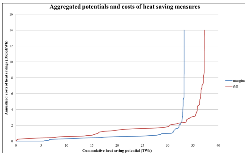
Figure 4. Cumulative potentials and marginal and full costs of heat savings without disaggregation on different building elements.
