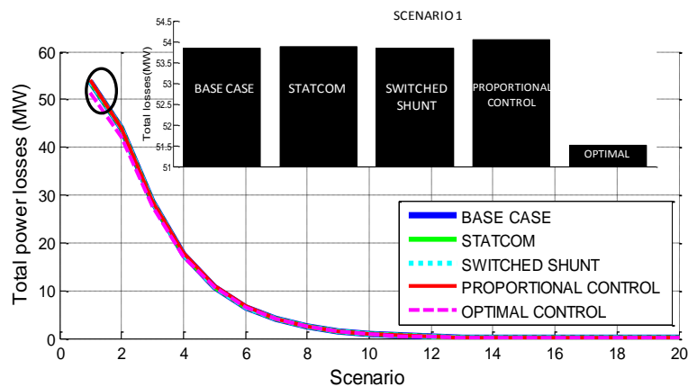
Figure 3.41: Power losses for the five cases under study in all the scenarios evaluated, providing a zoom analysis of the first scenario, network 1.
