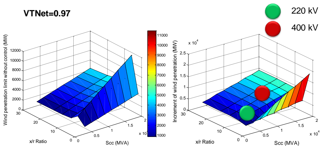
Figure 3.22: Wind penetration increment when VNet is 0.97 p.u.
