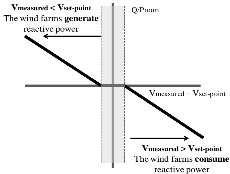
Figure 3.36: Reactive power required in order to provide voltage control in accordance with Spanish Operational Procedure
