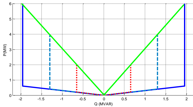
Figure 3.14: Extrapolated PQ curves
