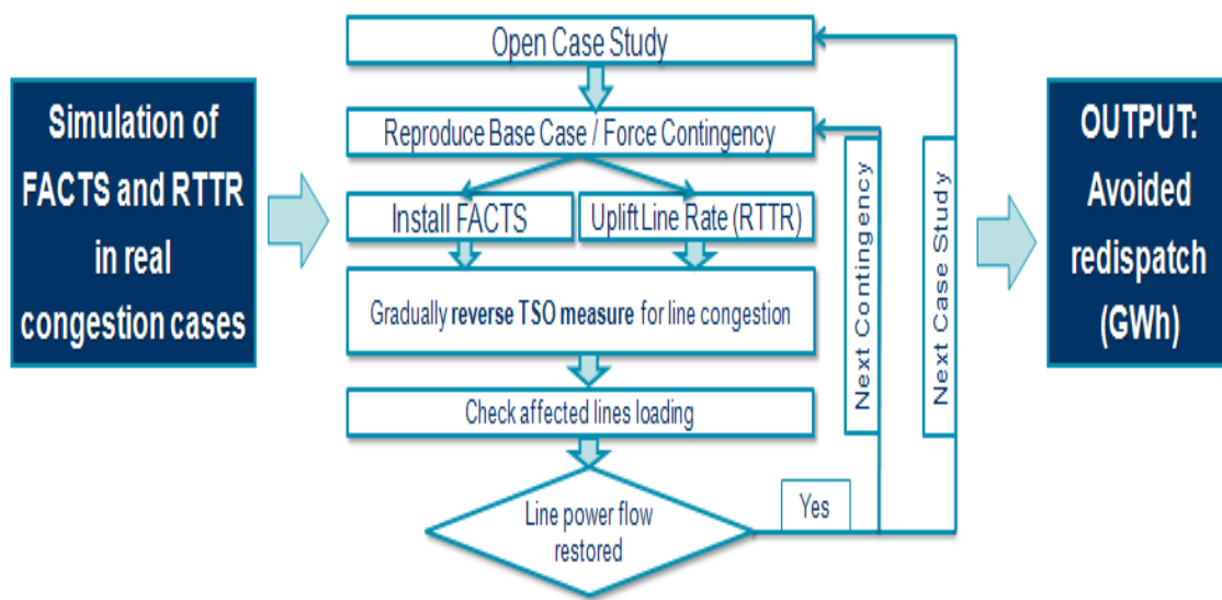
Figure 6.1: Python routine
