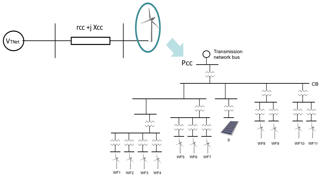
Figure 3.28: Harvesting network.
