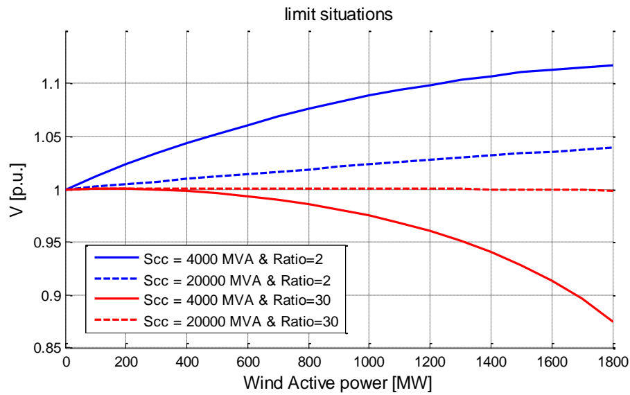
Figure 3.9: Short-circuit power (Sc) and x/r ratio impact on the PV curve
