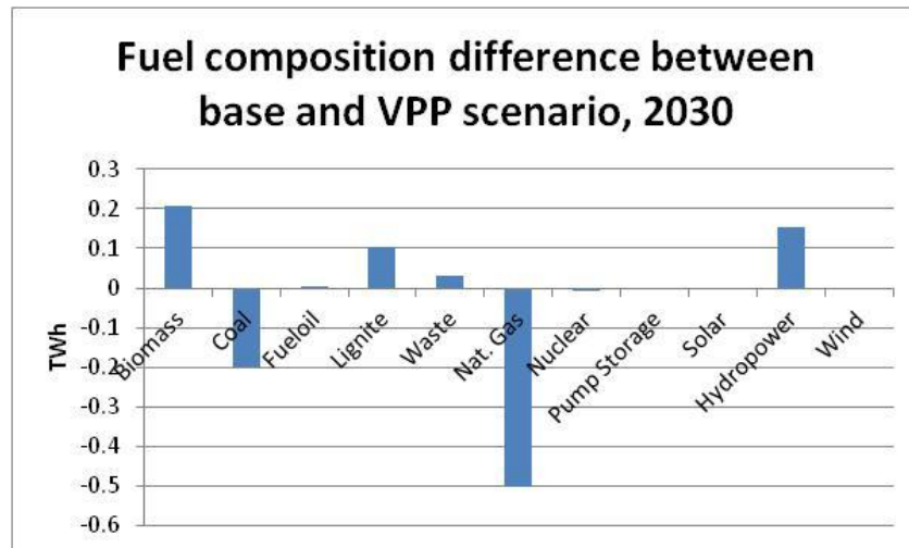
Figure 4.16: Fuel usage changes after VPP introduction
