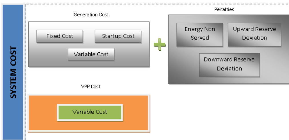
Figure 4.21: Global Objective Function of the Unit Commitment including VPP performance
