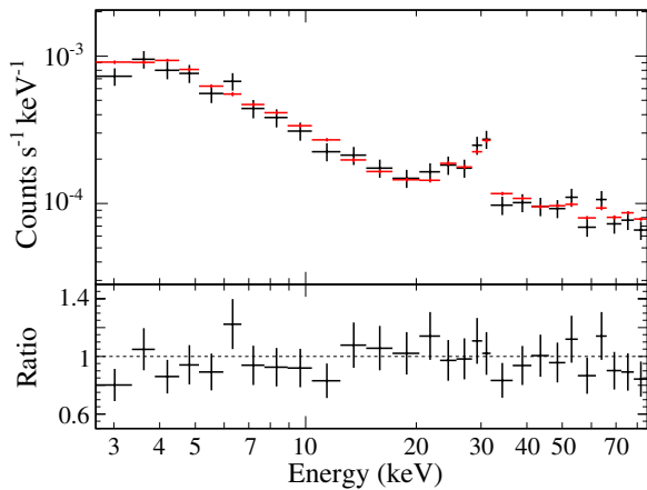
Figure 1. Comparison of (red) the background model produced by nuskybgd with (black) the actual blank-sky spectrum in the AE Aqr observation. The bottom panel shows the spectral ratio of the actual data to the model. (A color version of this figure is available in the online journal.)
