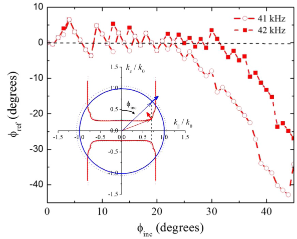
FIG. 2 (color online). Calculated propagating angle \phi_{\text{ref}} inside the hyperbolic material described in Fig. 1 as a function of the incident angle \phi_{\text{inc}} . The inset shows the equifrequency curves corresponding to airborne sound propagating in free space (circle of radius k_0 = 2\pi/\lambda_0 ) and inside a hyperbolic material with an infinite number of layers. k_{\parallel} and k_z are the components of the wave-vector parallel and perpendicular, respectively, to the stack of Plexiglas layers. In terms of wavelength, \lambda/D = 3.2 , \lambda/d_x = \lambda/d_y = 1.9 , and \lambda/d_z = 0.8 . The vertical dashed line is a guide for the eye indicating the conservation of k_{\parallel} .
