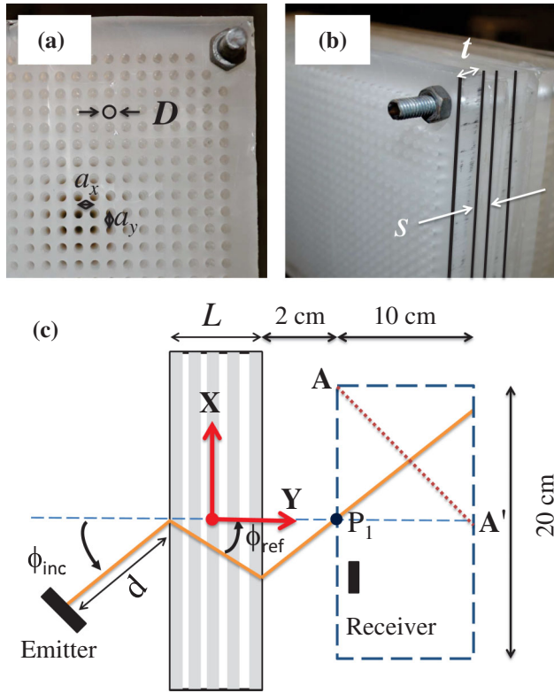
FIG. 1 (color online). (a) Frontal and (b) lateral views of the fabricated sample. It consists of a stack of holey Plexiglas plates with thickness t = 7.27 mm and separation s = 3.18 mm. The holes of diameter D = 2.7 mm are drilled in a square distribution with lattice period a_x = a_y = 4.54 mm. The hole periodicity along the normal is a_z = t + s = 10.45 mm. (c) Scheme (not to scale) of the experimental setup. The rectangle defined by the dashed lines defines the area scanned by the receiver-transducer. The sample represented consists of five holey plates (gray rectangles) with total thickness L .
