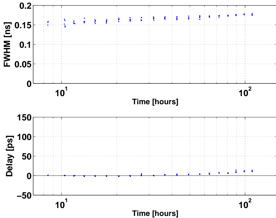
Figure 10. Pulse characteristics for the series of BG36 measurements presented in figure 9. Top: full width half maximum Bottom: temporal delay.
