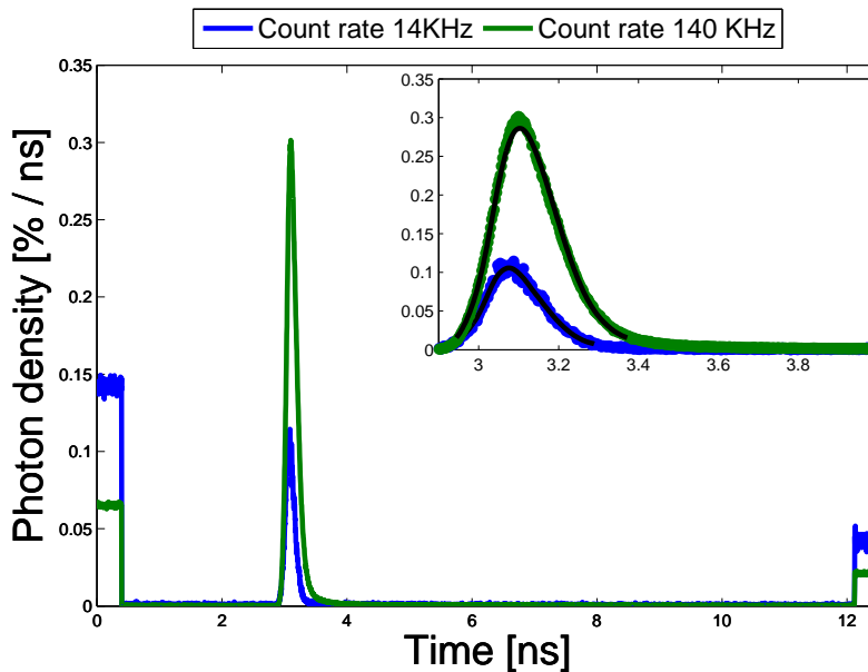
Figure 8. Example of PToF distributions for the BG36 phantom. The raw data is presented in the main plot, and the graph to the top right shows a zoom into the data with the fitted diffusion expression as black lines.
