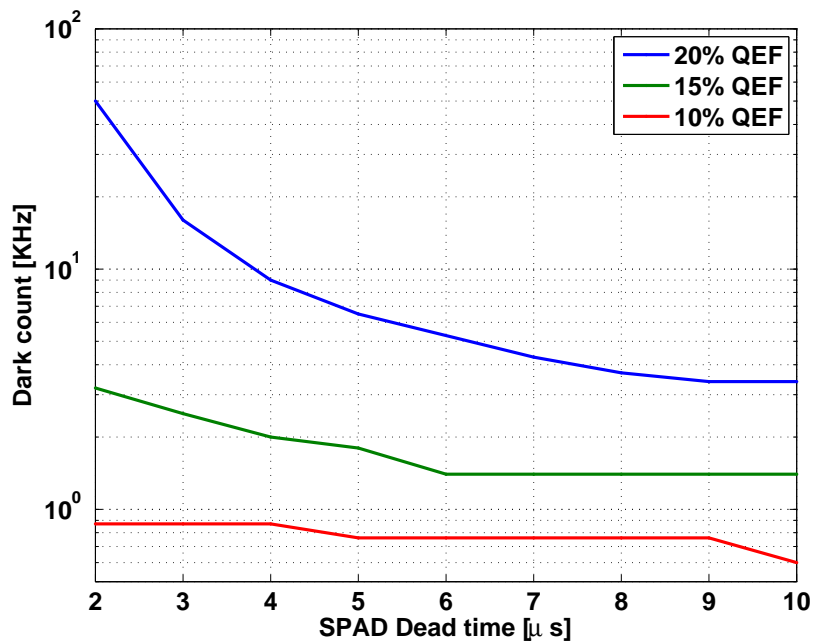
Figure 3. Measured dark counts as a function of dead time for different quantum efficiencies of the ID220.
