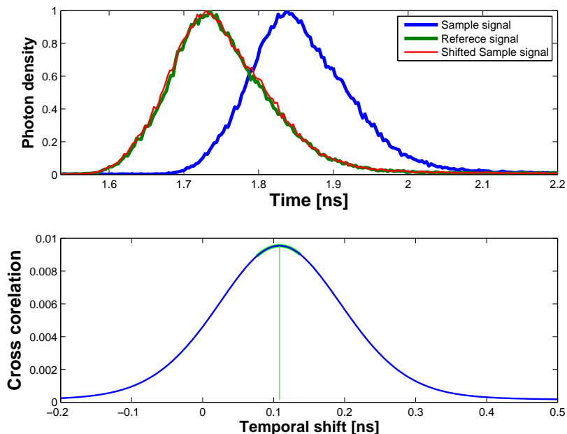
Figure 4. Example of how the temporal delay is calculated. Top: Examples of photon time-of-flight distributions and their overlap after using their cross correlation to estimating the temporal shift. Bottom: Cross correlation of the two profiles together with the fitted polynomial at the center. The position of the peak is marked with a vertical green line.
