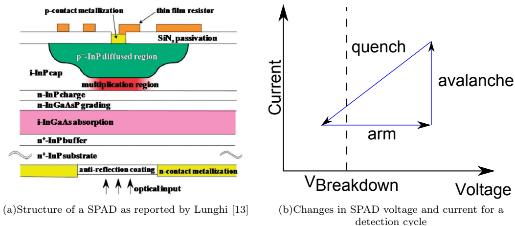
Figure 1. Illustration of the structure of an SPAD and the principle of its operation.
