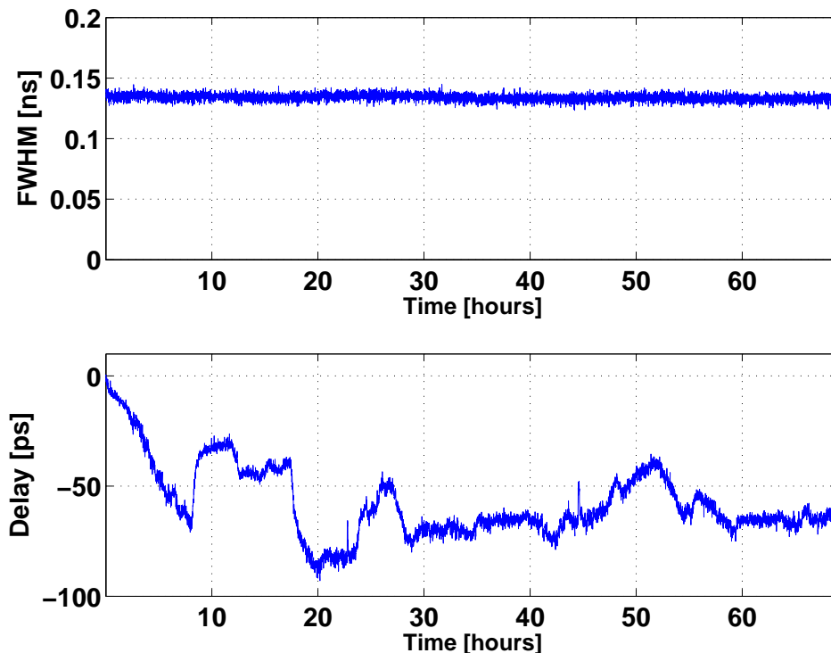
Figure 5. Time stability of the light source. Top: Measured full width half maximum of the PToF distribution. Bottom: Measured delay compared to the start point.
