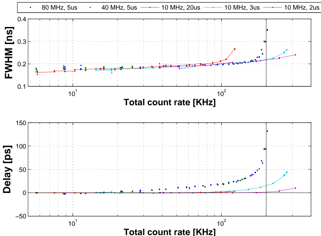
Figure 7. Instrument characteristics for different combinations of light source repetition rate and dead time, legend notes the repetition rate and dead time. Top: Absolute value for FWHM vs. count rate. Bottom: Measured delay relative to the 10 MHz value.
