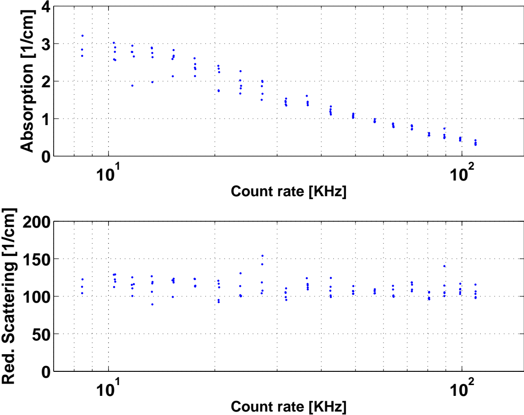
Figure 9. Deduced optical properties for a BG36 color glass phantom as a function of count rate, Top: Absorption Bottom: Reduced scattering
