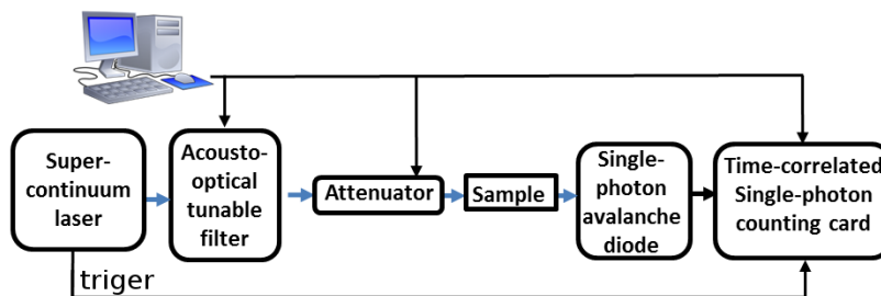
Figure 2. A schematic of the photon time-of-flight spectrometer. The black lines are electronic signals, and blue are optical.
