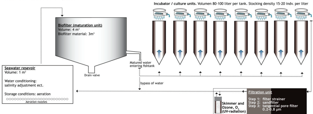
Figure 15. Schematic principle of matured water RAS system for European eel larvae culture. See description in text.
