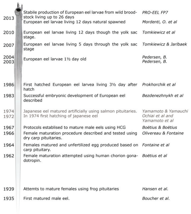
Figure 3. Time line showing major events in the progress of producing larvae of European eel, Anguilla anguilla in captivity. Grey text indicates milestones in Japanese eel, A. japonica reproduction studies.
