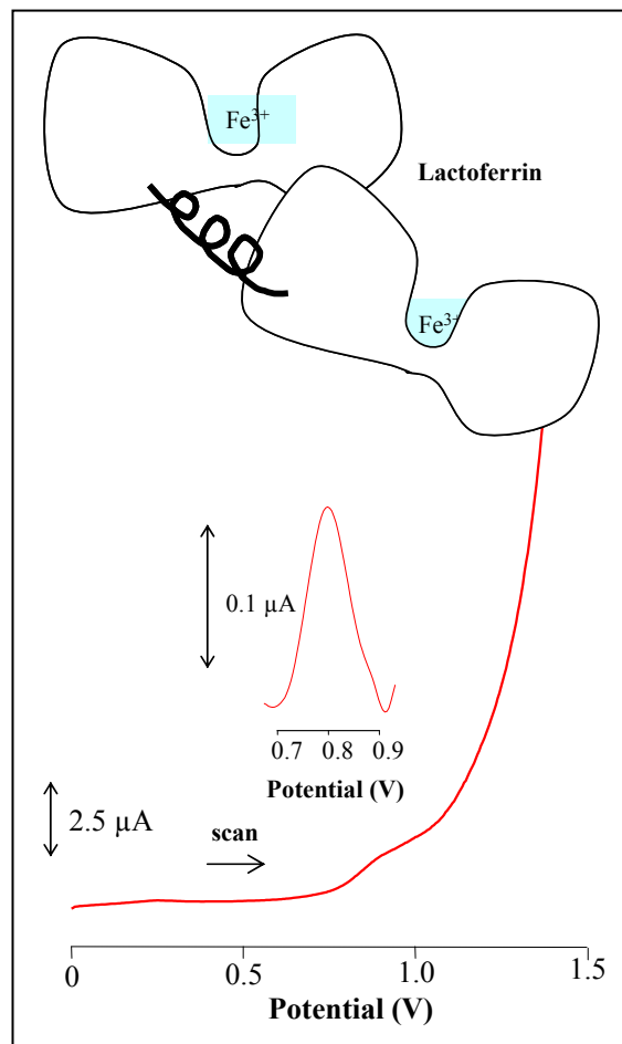
Figure 7. The typical linear sweep voltammogram of lactoferrin measured at carbon paste electrode. Lactoferrin concentration was 1 µg/ml, Acetate buffer (0.1 M CH 3 COOH + 0.1 M CH 3 COONa, pH 5.0) was used as the supporting electrolyte. The linear sweep voltammetric parameters were as follows: initial potential of 0 V, end potential 1.5 V, step potential 5 mV, scan rate 50 mV/s. Experimental data were processed using smoothing and baseline correction.
