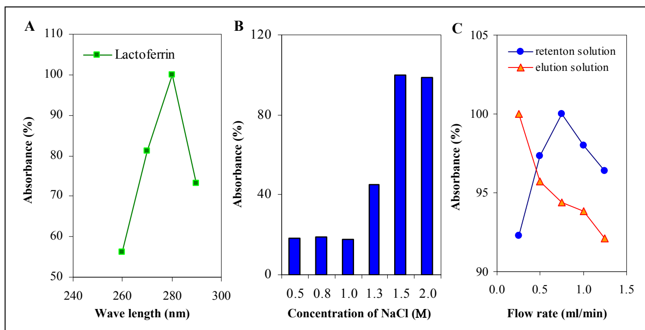
Figure 4. The influence of (A) wave length, (B) ionic strength of the elution solution (NaCl) and (C) flow of the elution solution on height of the lactoferrin signal.
