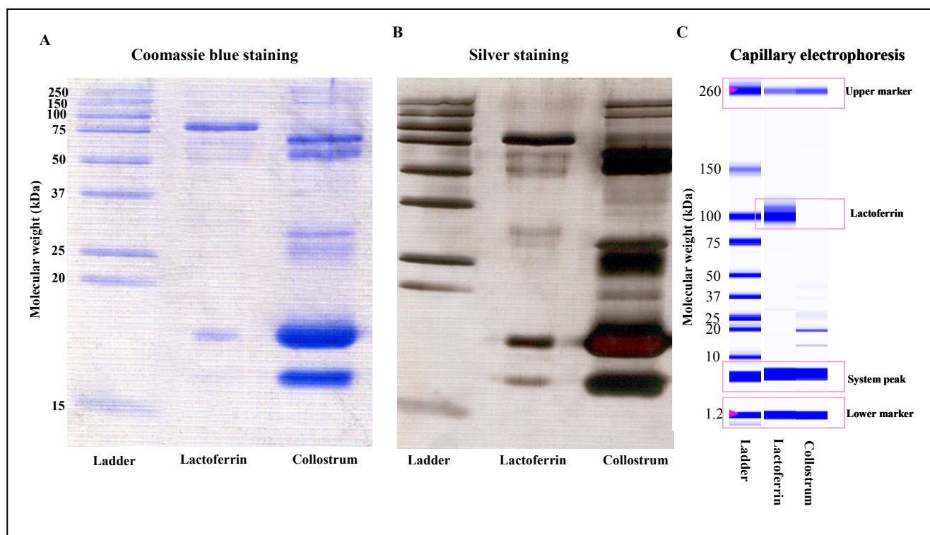
Figure 2. SDS-PAGE with (A) Coomassie blue staining or (B) Silver staining and (C) Experion capillary electrophoresis of ladder, lactoferrin standard (100 \mu\text{g}/\text{ml} ) and milk sample
