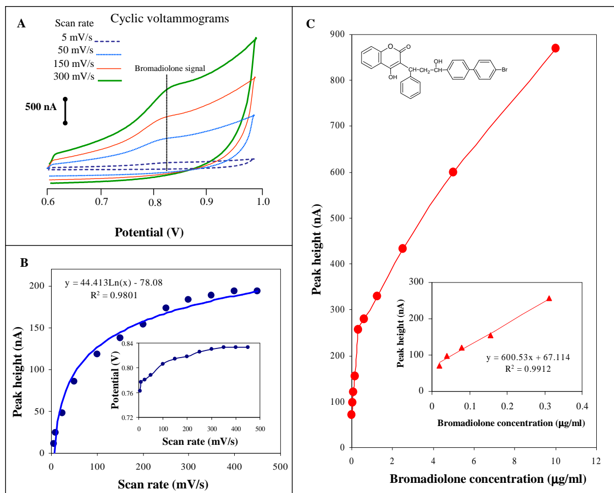
Figure 3. The electrochemical analysis of bromadiolone using cyclic voltammetry. (A) Cyclic voltammograms of bromadiolone (1 \mu\text{g/ml} ) at scan rate of 5, 50, 150, and 300 mV/s. (B) Dependence of the height and position of potential of the bromadiolone signal on the scan rate. (C) Variation in the height of the bromadiolone signal on the concentration at a scan rate of 300 mV/s. Parameters of measurement: 0.2 M acetate buffer (pH 4.0), in the potential range from 0.6 to 1 V, potential step: 2.4 mV, experiments were carried out at room temperature.
