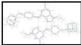
Fig. 1. ORTEP plot of the asymmetric unit with atoms represented as 50% probability ellipsoids (H-bonds are denoted as dashed lines).
