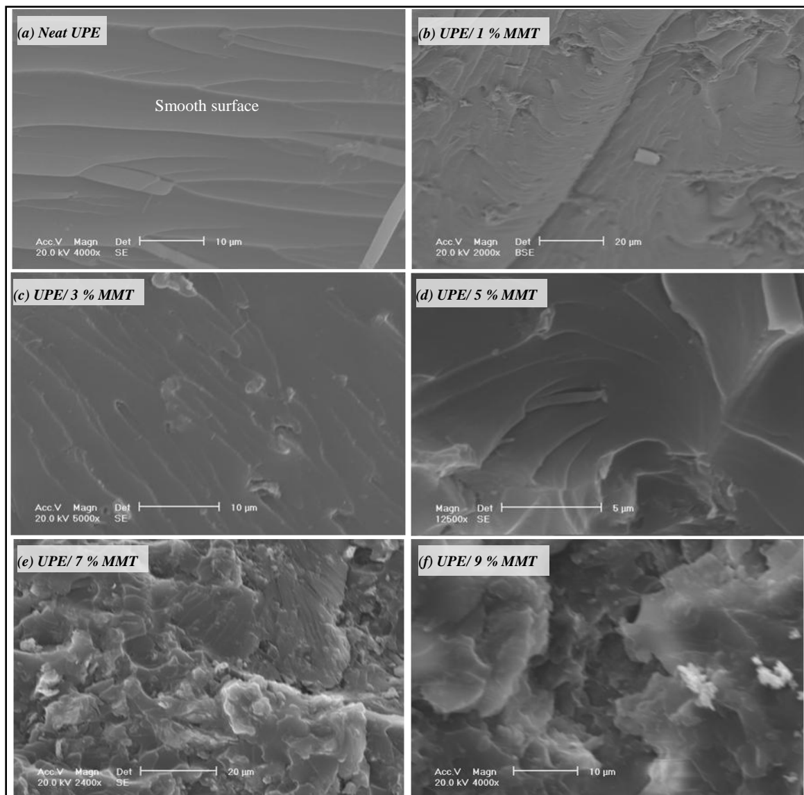
Fig. 5 SEM images showing the failure mechanisms of fracture surface obtained from the CT specimens for the neat UPE and UPE-based different MMT nanocomposites.
