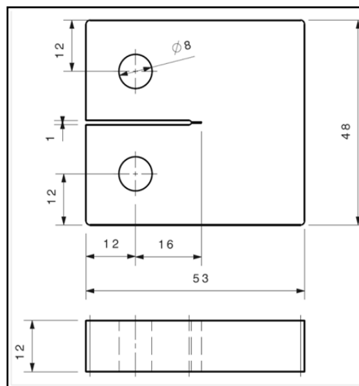
Fig. 1 Dimensions of the compact tension (CT) specimen.
