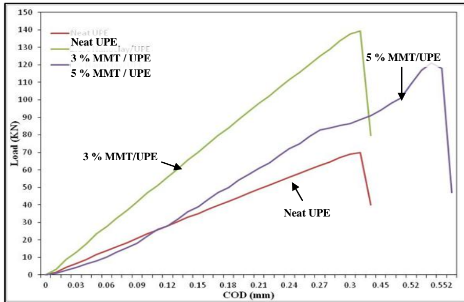
Fig. 3 The typical loads versus crack opening displacement (COD) curves.
