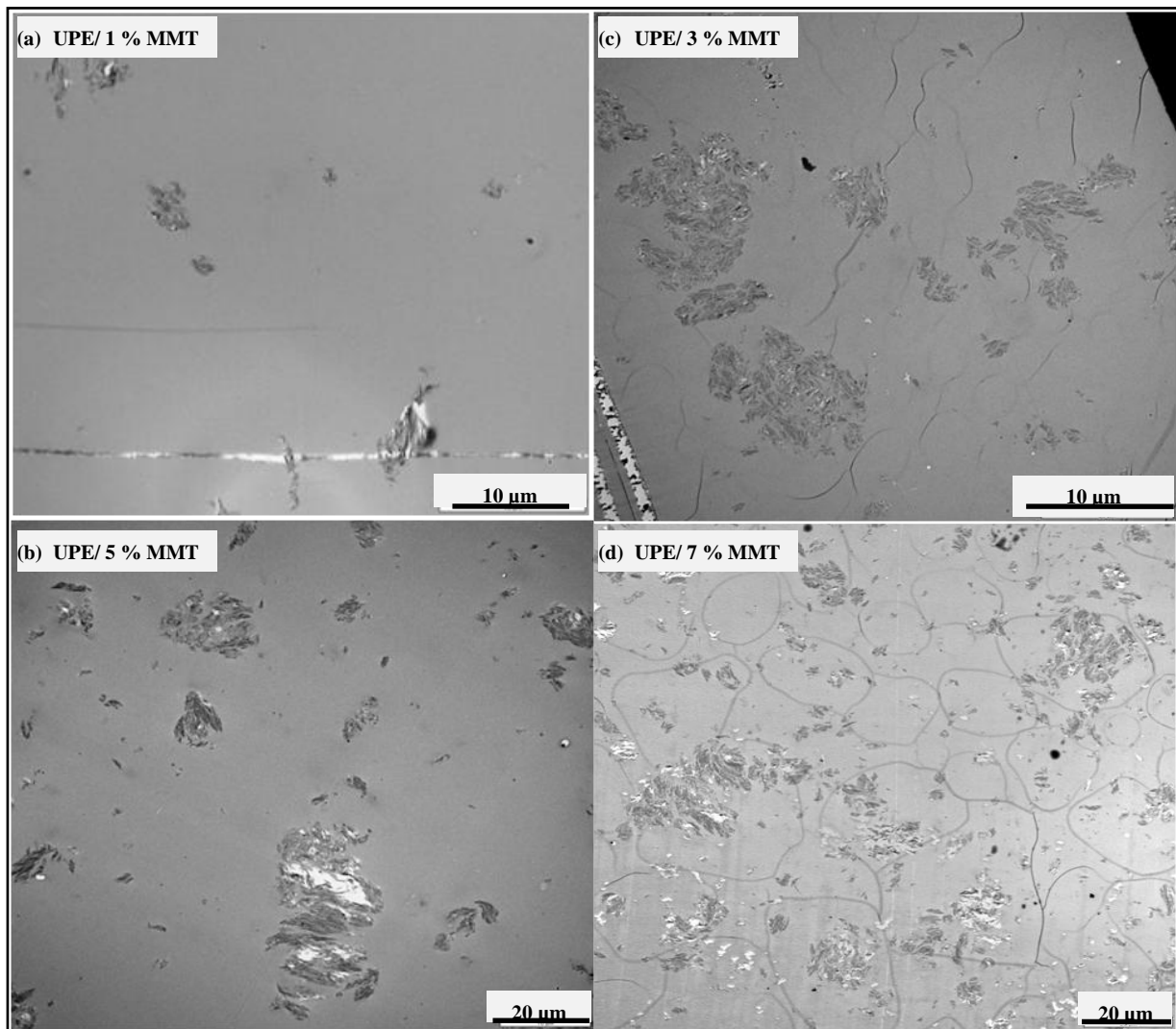
Fig. 2 TEM photomicrographs of UPE-based different MMT nanocomposites.
