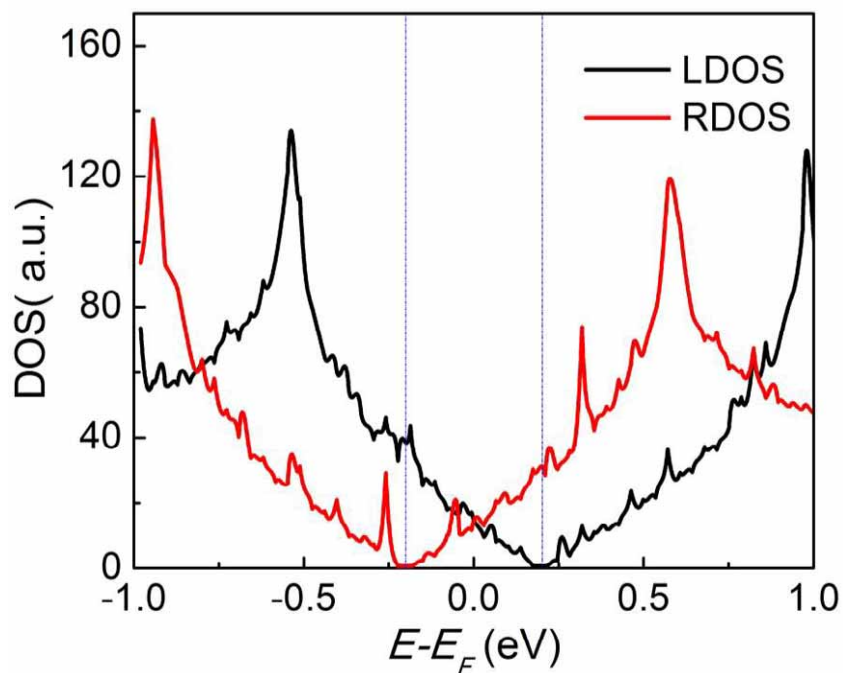
Figure S1. Density of states (DOS) of the left (LDOS) and right (RDOS) electrodes under the bias voltage of 0.4 V for the two-probe \alpha -graphyne device. The chemical potentials of left and right electrodes ( u_L and u_R ) are separated by eV_b = 0.4 eV.
