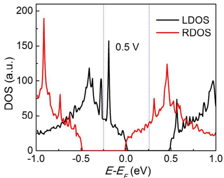
Figure S5. Density of states (DOS) of the left (LDOS) and right (RDOS) electrodes under the 0.5 V bias voltage for the two-probe \gamma -graphyne sheet device. The chemical potentials of left and right electrodes ( u_L and u_R ) are separated by eV_b = 0.5 eV.
