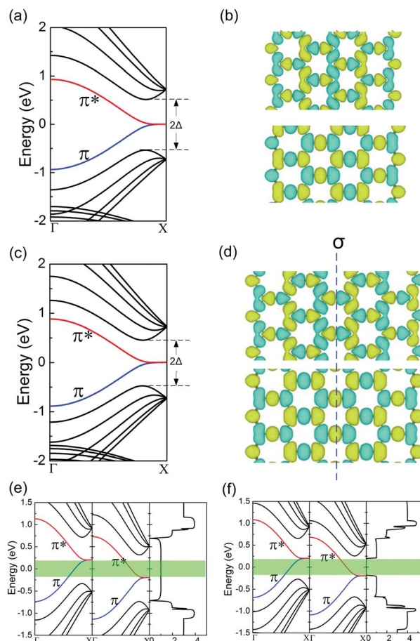
Fig. 4 (a) Band structure around the Fermi level and (b) \Gamma -point wave functions of \pi and \pi^* subbands for 5- \alpha -ZGyNR. (c) Band structure around the Fermi level and (d) \Gamma -point wave functions of \pi and \pi^* subbands for 6- \alpha -ZGyNRs. (e) Band structures for the left and right electrodes, and the transmission spectrum of 5- \alpha -ZGyNRs under 0.4 V bias voltage (highlighted by the green bar). (f) Band structures for the left and right electrodes, and the transmission spectrum of 6- \alpha -ZGyNR under 0.4 V bias voltage. The yellow and blue colors indicate opposite signs of the wave function.
