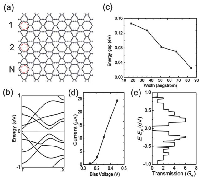
Fig. 6 (a) Atomic structure of 1D armchair \beta -GyNRs. (b) Computed band structure of 2- \beta -AGyNR. (c) The variation in the band gap E_g of the \beta -AGyNRs as a function of ribbon width. (d) The I - V_b curve and (e) the transmission spectrum at the zero-bias voltage for the two-probe 2- \beta -AGyNR device.
