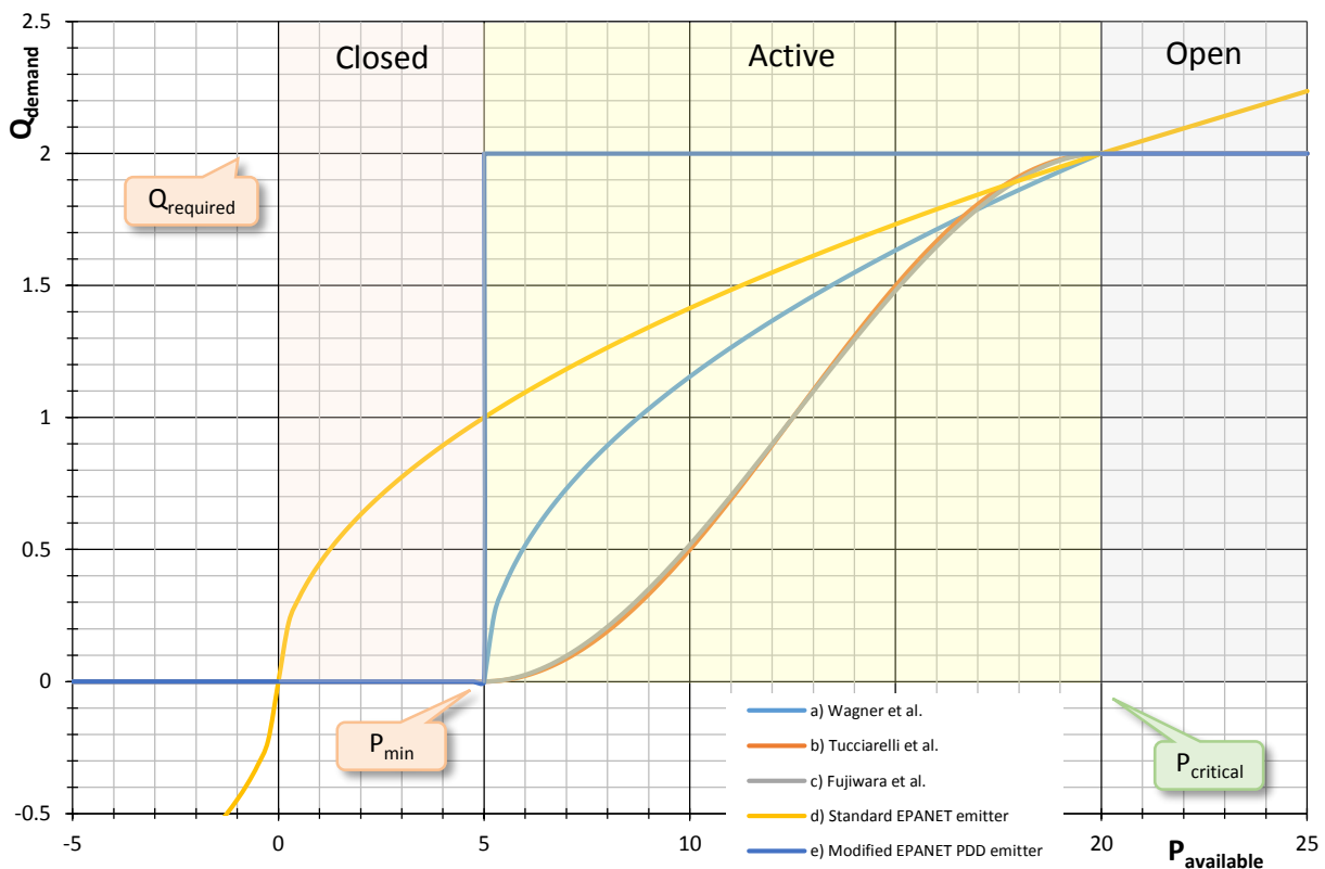
Figure 1: Head/Flow relationship for a Pressure Driven Demand node as implemented in EPANETpdd
