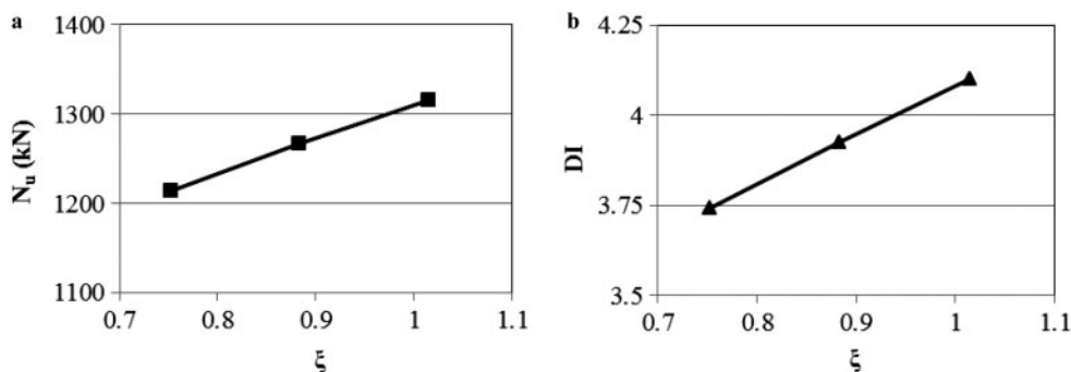
Fig. 11. Confinement effect of steel wall for the columns ( \theta = 1.65^\circ & t = 3 \text{ mm}, 3.5 \text{ mm}, \text{ and } 4 \text{ mm} ): (a) on ultimate axial load capacity, (b) on ductility
