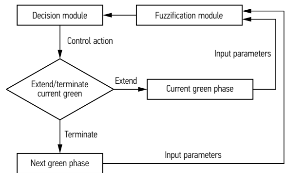
Fig. 3. System control architecture
