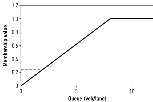
Fig. 1. Fuzzy set of ‘extend green signal’
