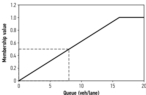
Fig. 2. Fuzzy set of ‘terminate green signal’
