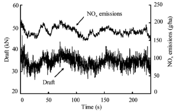
Fig. 2. Dependencies of traction force and NOx emissions and their interrelation in real-time soil preparation work (Li et al. 2006)
