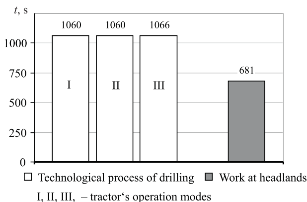
Fig. 5. Distribution of drilling process times between operating modes
