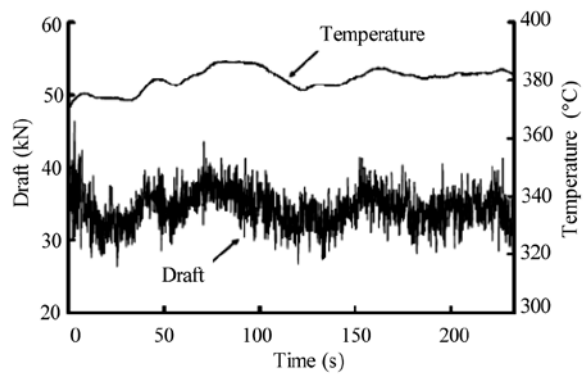
Fig. 3. Dependencies of traction force and combustion gas temperatures and their interrelation in real-time soil preparation work (Li et al. 2006)
