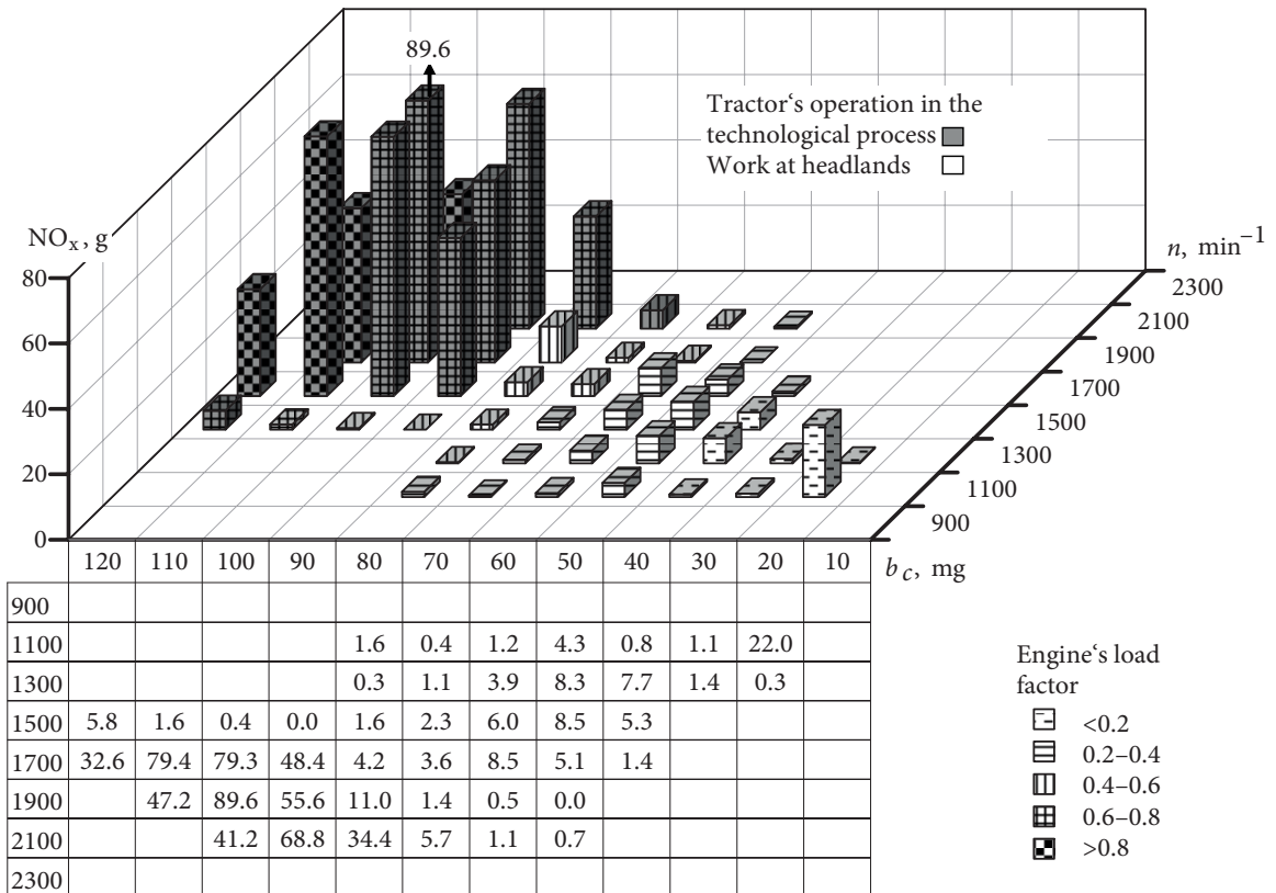
Fig. 12. Distribution of NO x emissions during the test period of drilling (3867 s) in the modes of engine speed (n) and cyclic fuel injection quantity (b)
