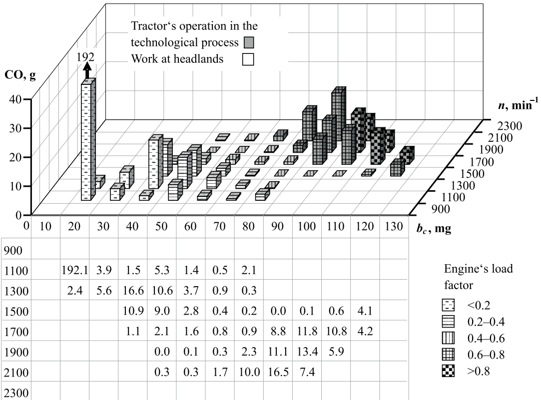
Fig. 10. Distribution of CO emissions during the test period of drilling (3867 s) in the modes of engine speed ( n ) and cyclic fuel injection quantity ( b_c )
