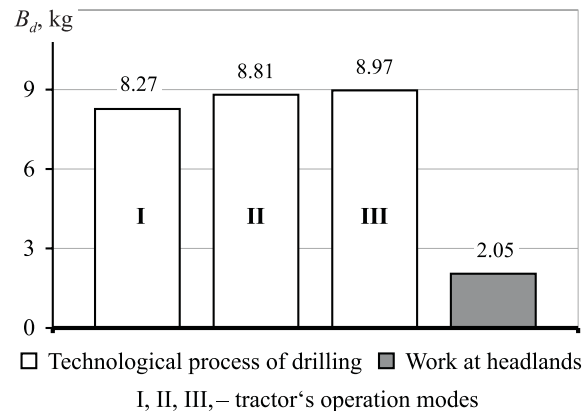
Fig. 7. Distribution of fuel consumption during the process of drilling test (3867 s) by the operating modes
