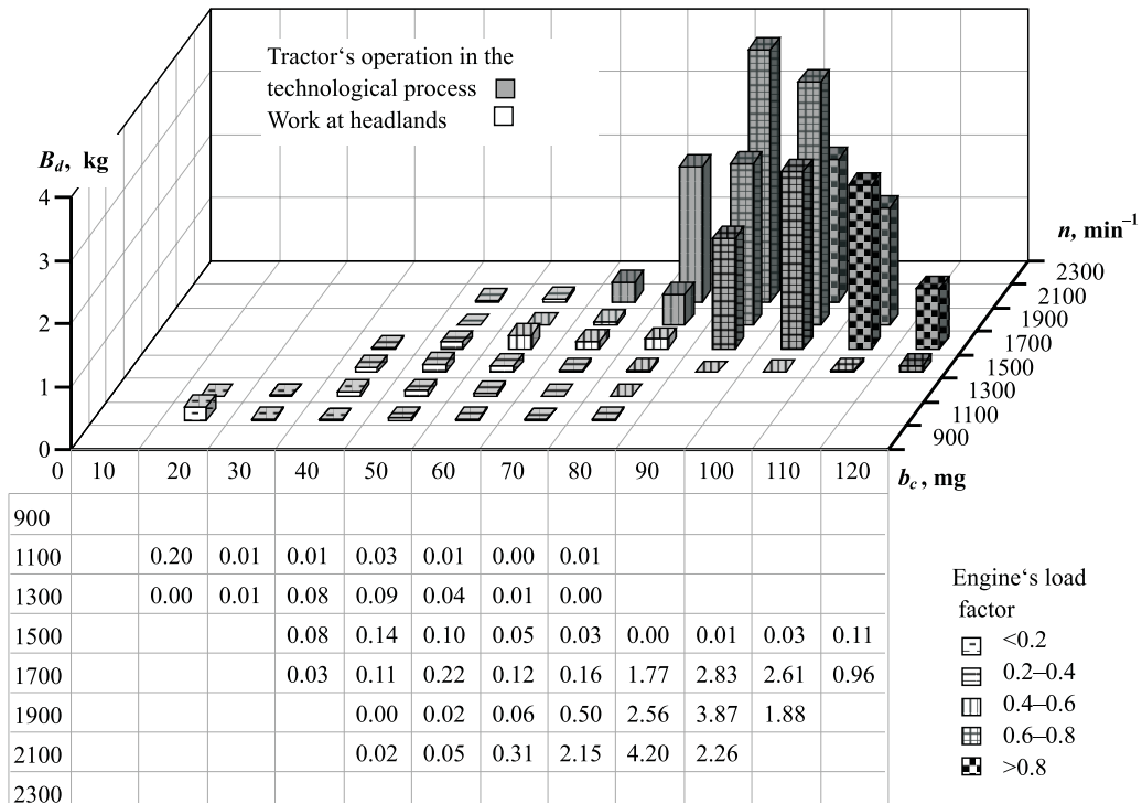
Fig. 8. Distribution of unit's fuel consumption during the test period (3867 s) in the modes of engine speed ( n ) and cyclic fuel injection quantity ( b_c )
