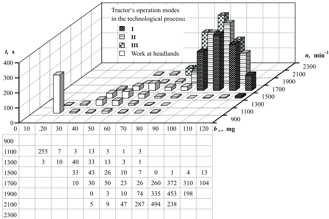
Fig. 6. Distribution of unit's working time period (3867 s) in the modes of engine speed ( n ) and cyclic fuel injection quantity ( b )
