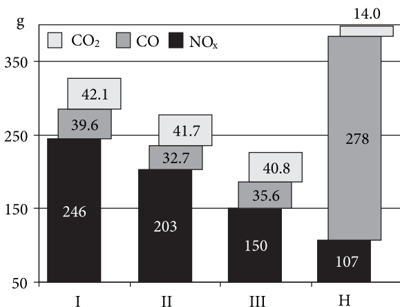
Fig. 9. Distribution of emitted combustion components CO, CO 2 and NO x during the test period (3867 s) in the drilling process by operating modes; I, II, III – tractor's operation modes, H – mode at headland
