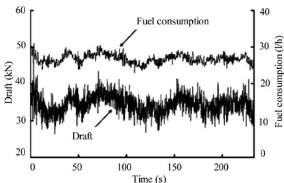
Fig. 1. Dependencies of traction force and fuel consumption and their interrelation in real-time soil preparation work (Li et al. 2006)
