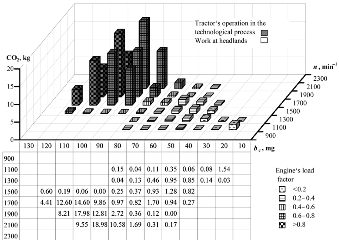
Fig. 11. Distribution of CO 2 emissions during the test period of drilling (3867 s) in the modes of engine speed ( n ) and cyclic fuel injection quantity ( b_c )
