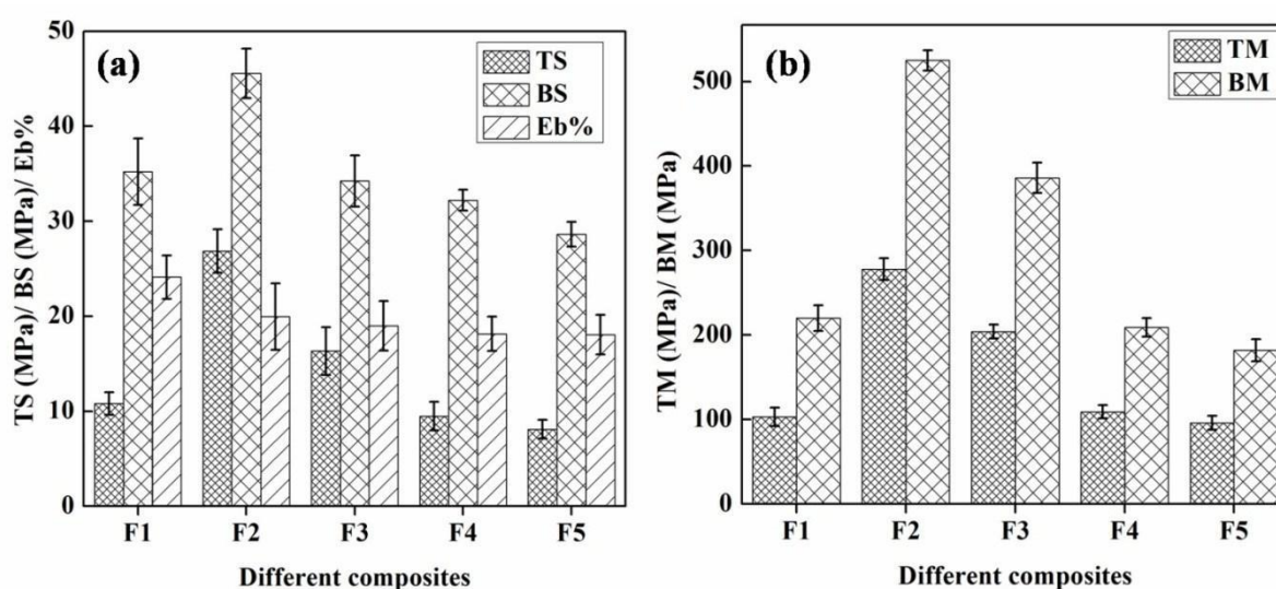
Figure 6. Mechanical properties (a) tensile strength, bending strength and elongation at break (Eb%) and (b) tensile and bending modulus of the composites.
