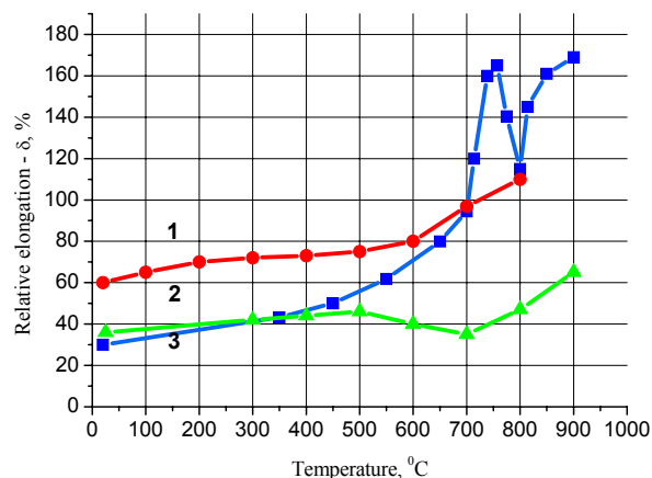
Fig.2. Temperature dependencies of plastic properties of high-purity hafnium (1), hafnium iodide (2) and hafnium HFE-1 (3).
