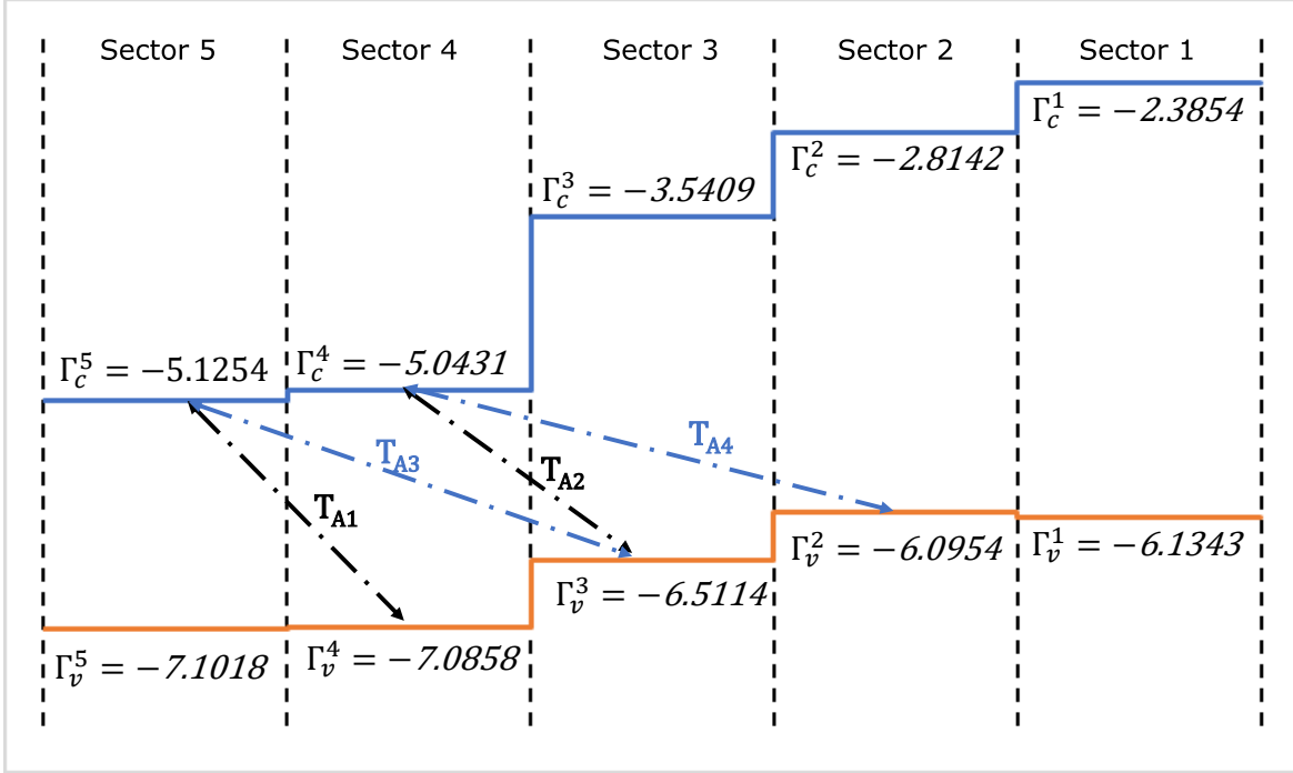
Figure 41 Electron Band Diagram for \text{InC}_x\text{N}_{1-x} at point \Gamma .
