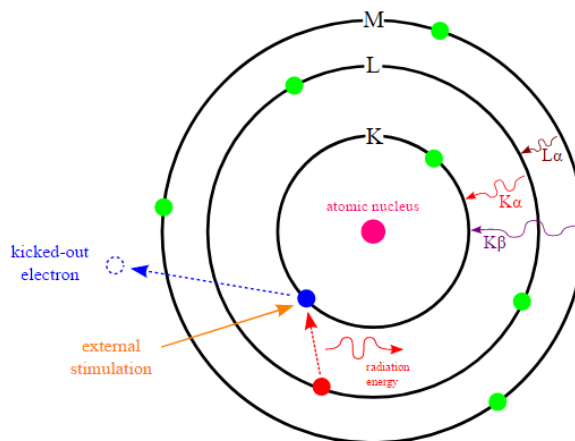
Figure 10 Schematic on how an electron is removed from the K-Shell [33]
