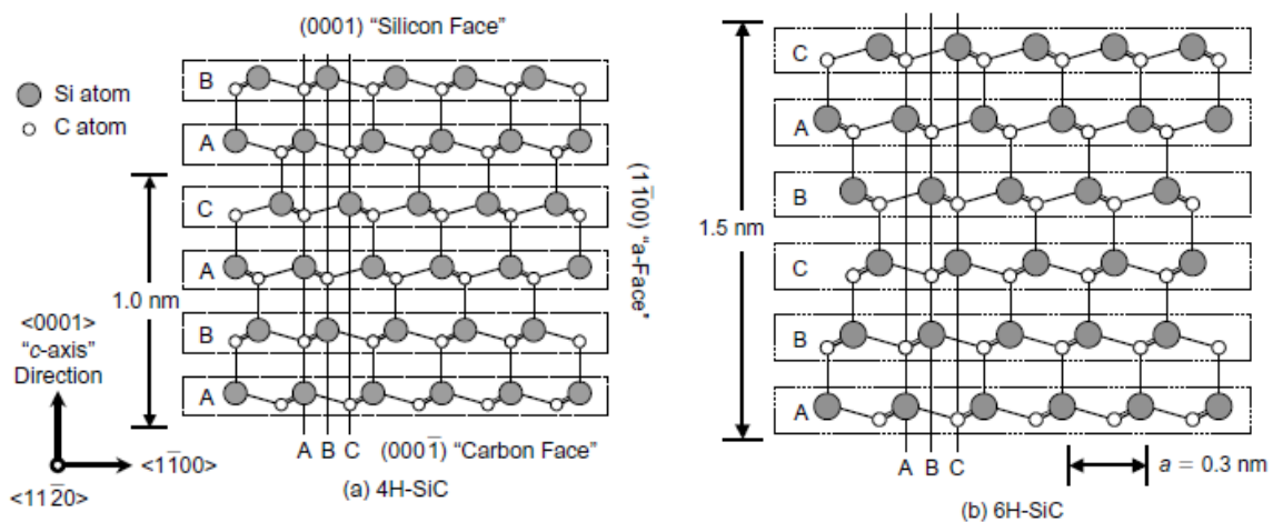
Figure 6 Cross section of (a) 4H-SiC and (b) 6H-SiC atomic crystal structure showing direction and surface faces [25]
