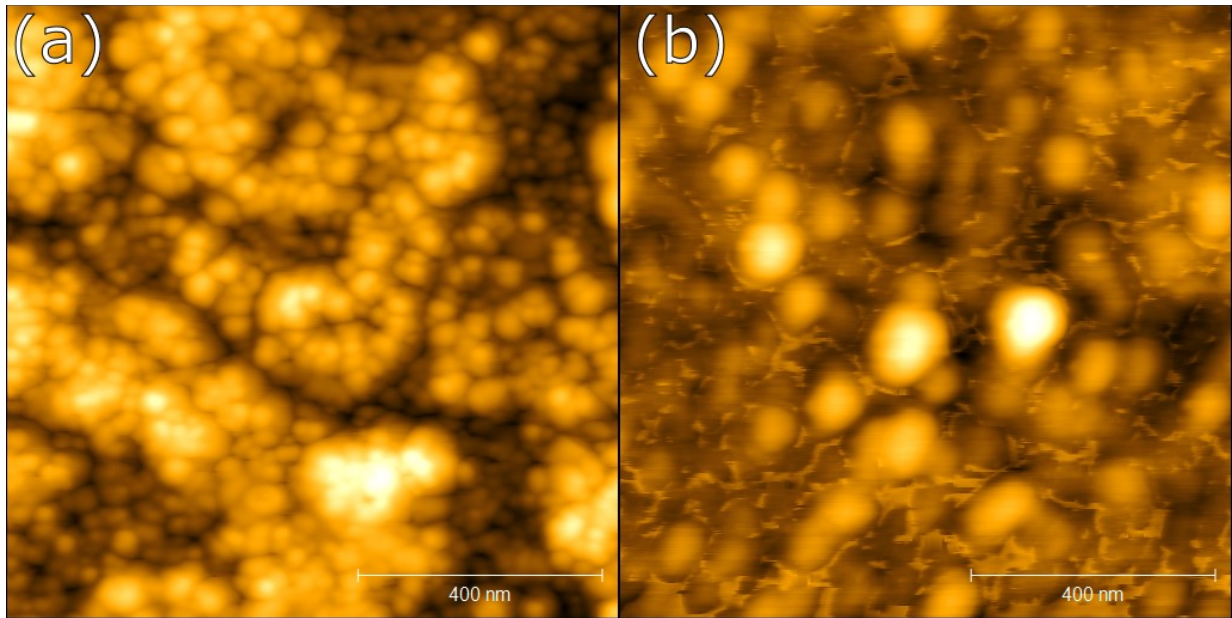
Figure 27 AFM Measurements for GaN (a) Growth 19, (b) Growth 10
