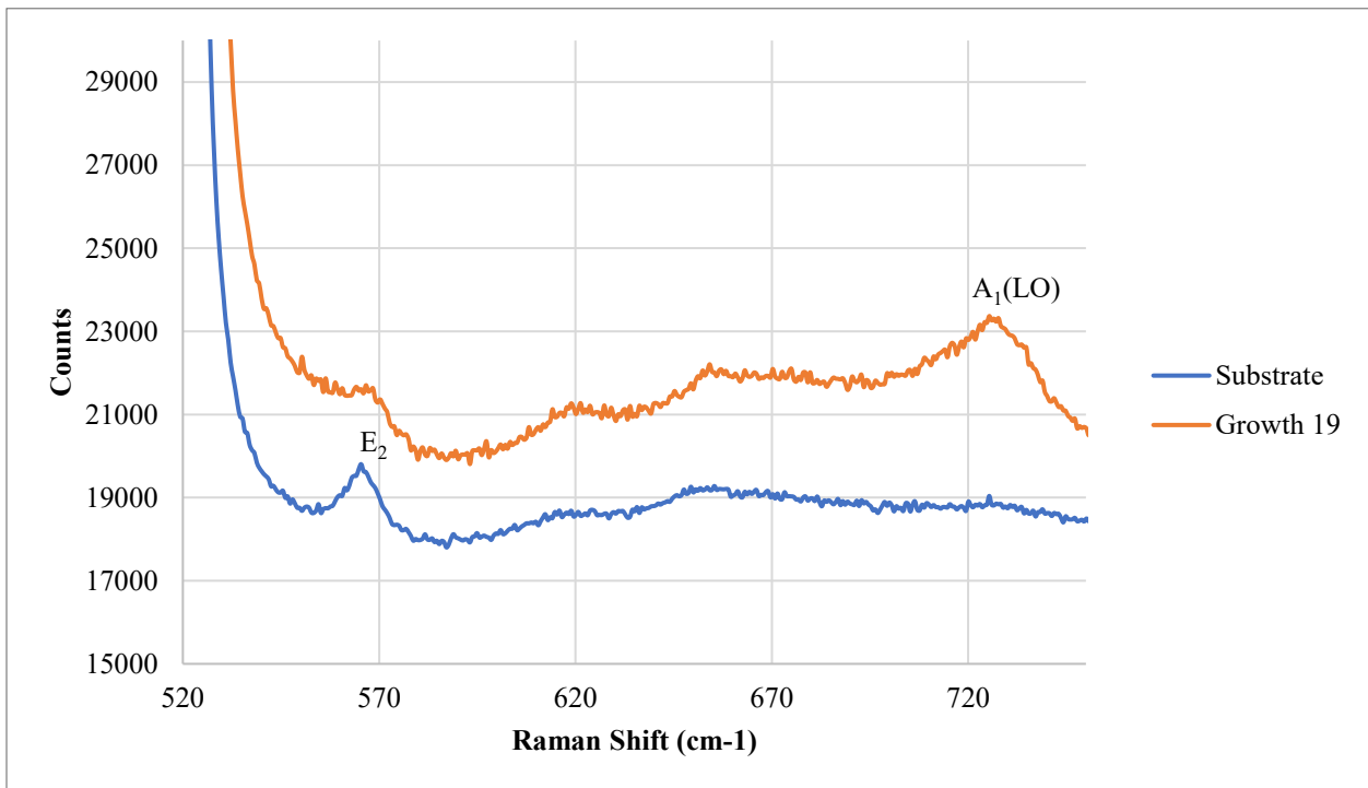
Figure 28 Raman measurements for growth 19 as compared to the substrate
