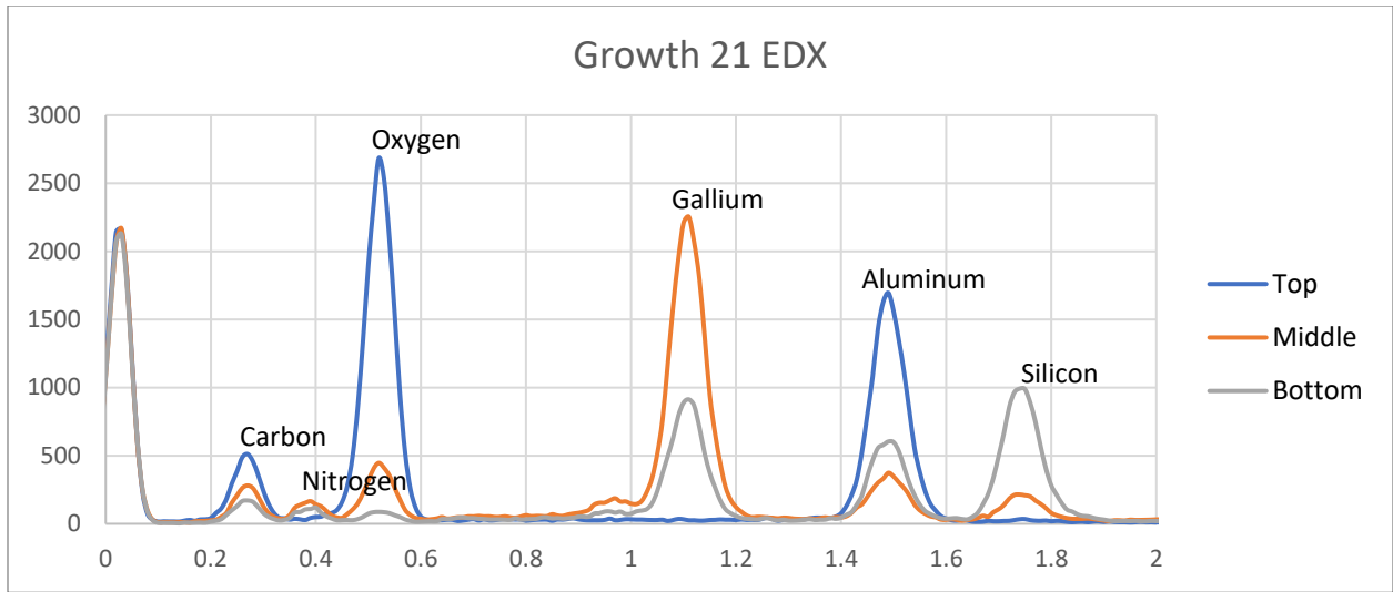
Figure 24 EDX graph for growth 21
