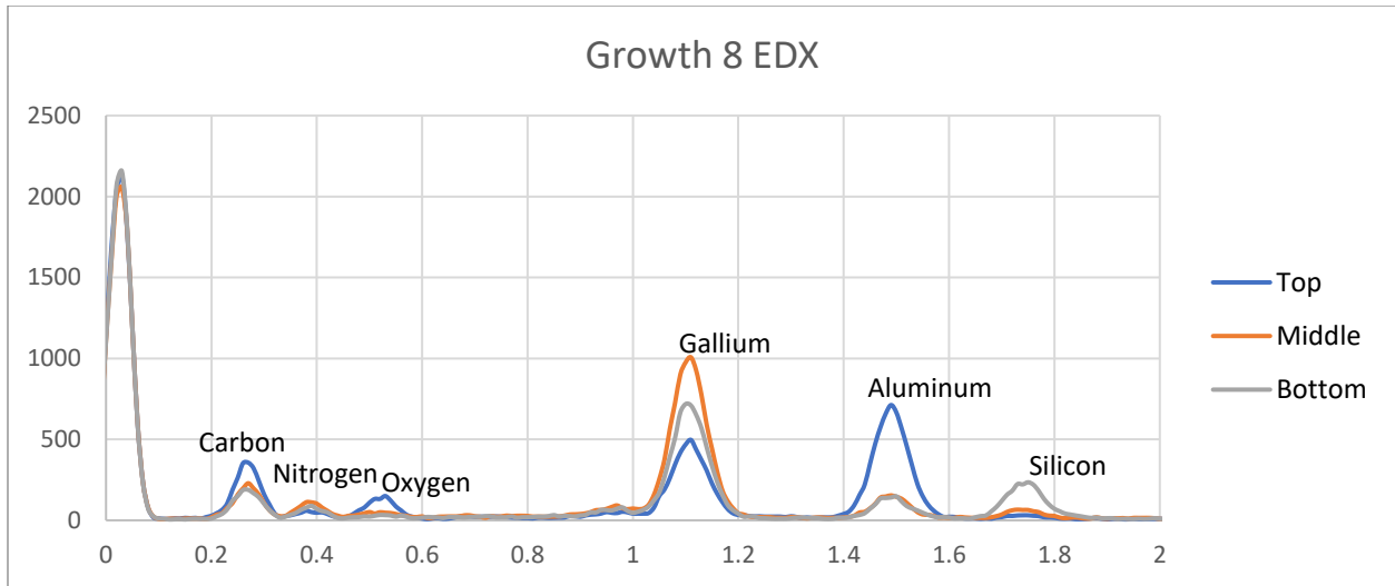
Figure 22 EDX graph for growth 8
