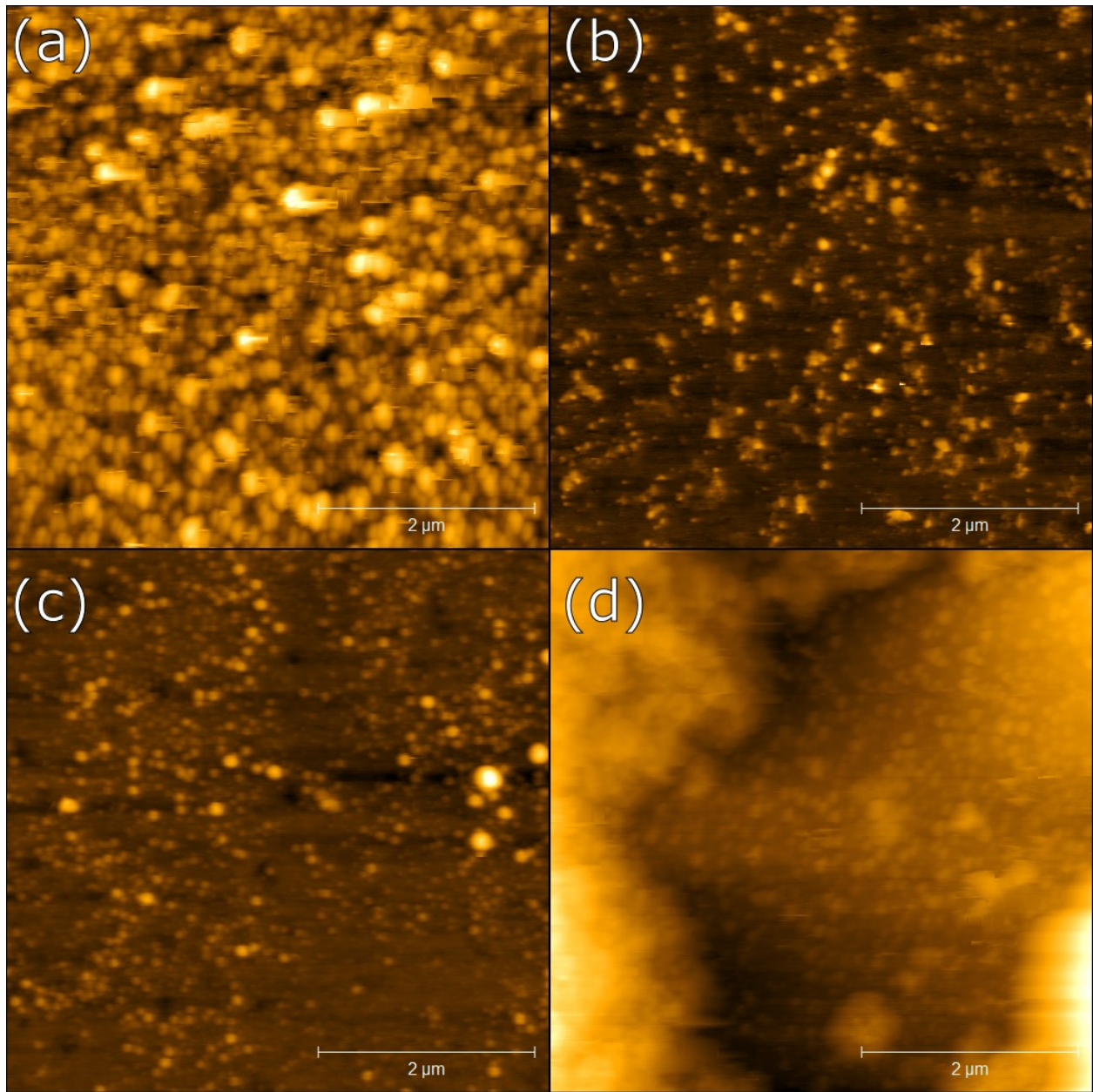
Figure 25 AFM scans of (a) Growth 3, (b) Growth 8, (c) Growth 17 and (d) Growth 21
