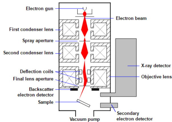
Figure 8 Schematic of a typical SEM beam and electron gun. [31]
