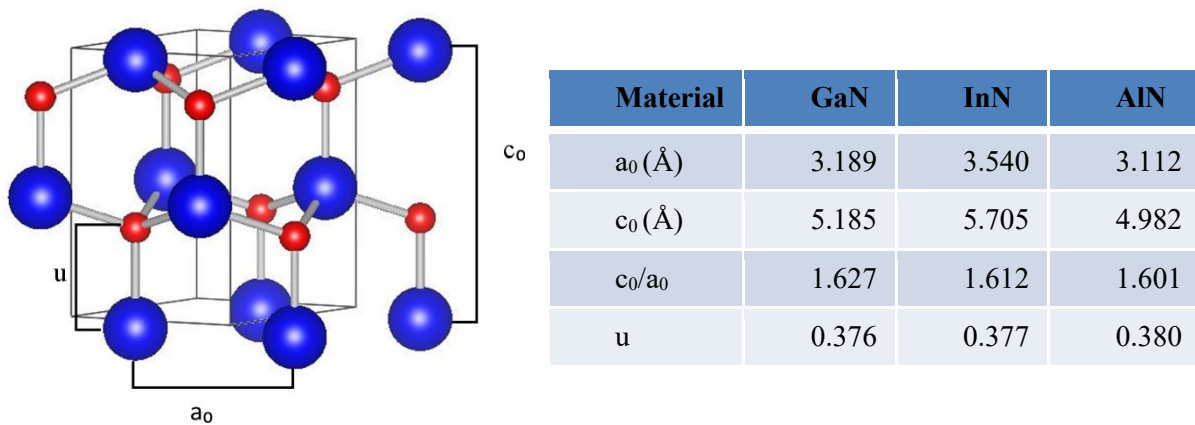
Figure 4 Unit cell of wurtzite crystal showing the tetrahedral structure along with the physical dimensions of the III-nitrides.
