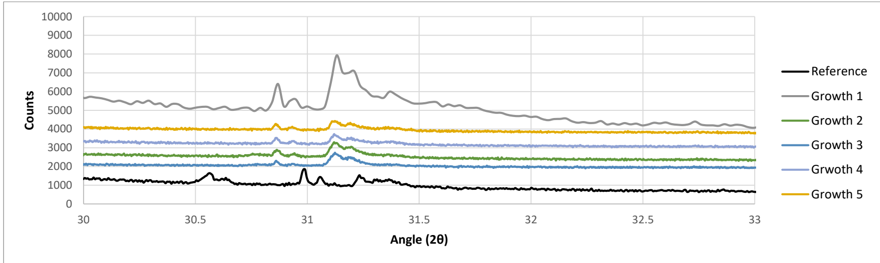
Figure 37 XRD scans of InN
