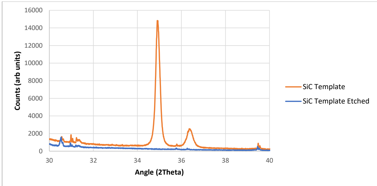
Figure 18 XRD plot of the template vs the etched template after removal of all the GaN
