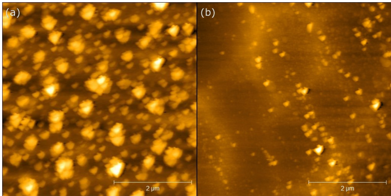
Figure 19 (a) SiC template before etching (b) SiC Template after etching
