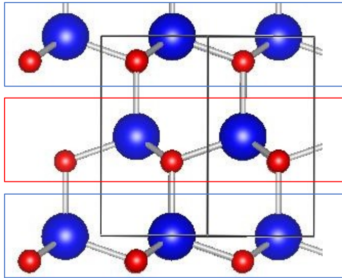
Figure 5 Stacking in a wurtzite crystal in the ABABAB format. The blue outline is A and the red outline is B
