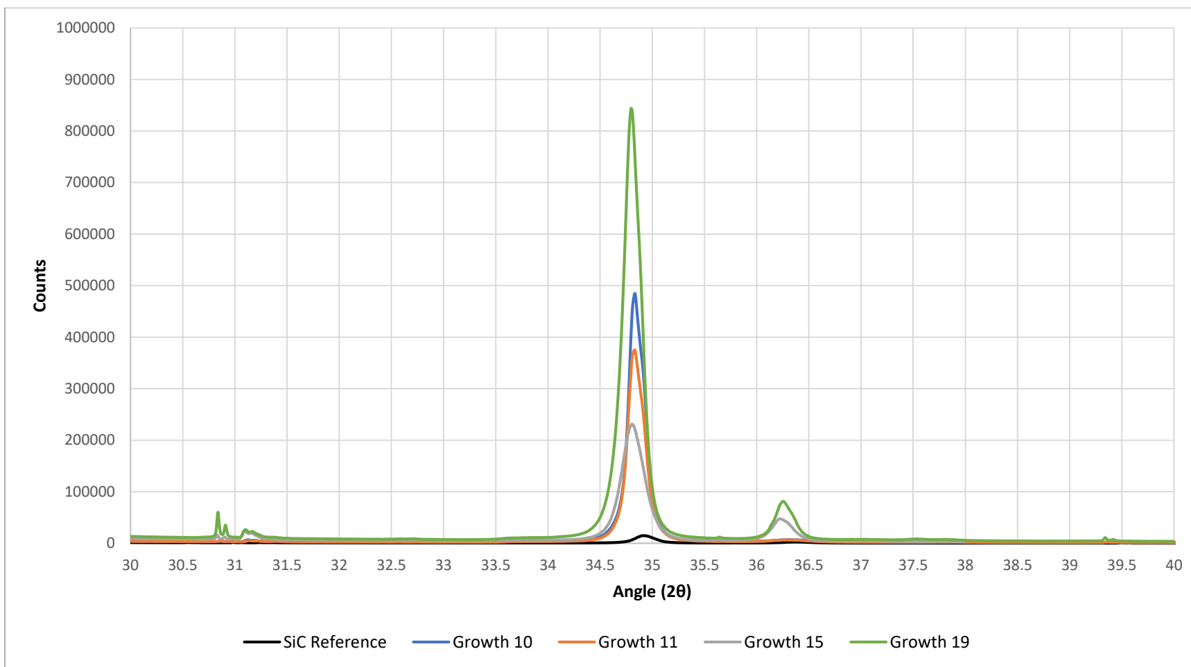
Figure 32 GaN XRD Plots
