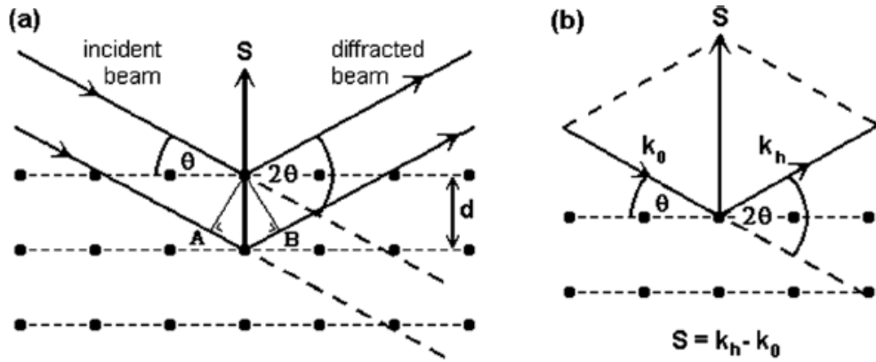
Figure 7 (a) Bragg's condition for x-ray diffraction and (b) relationship between incident ( k_0 ), diffracted ( k_h ) and the scattering vector S with respect to the crystal. [30]
