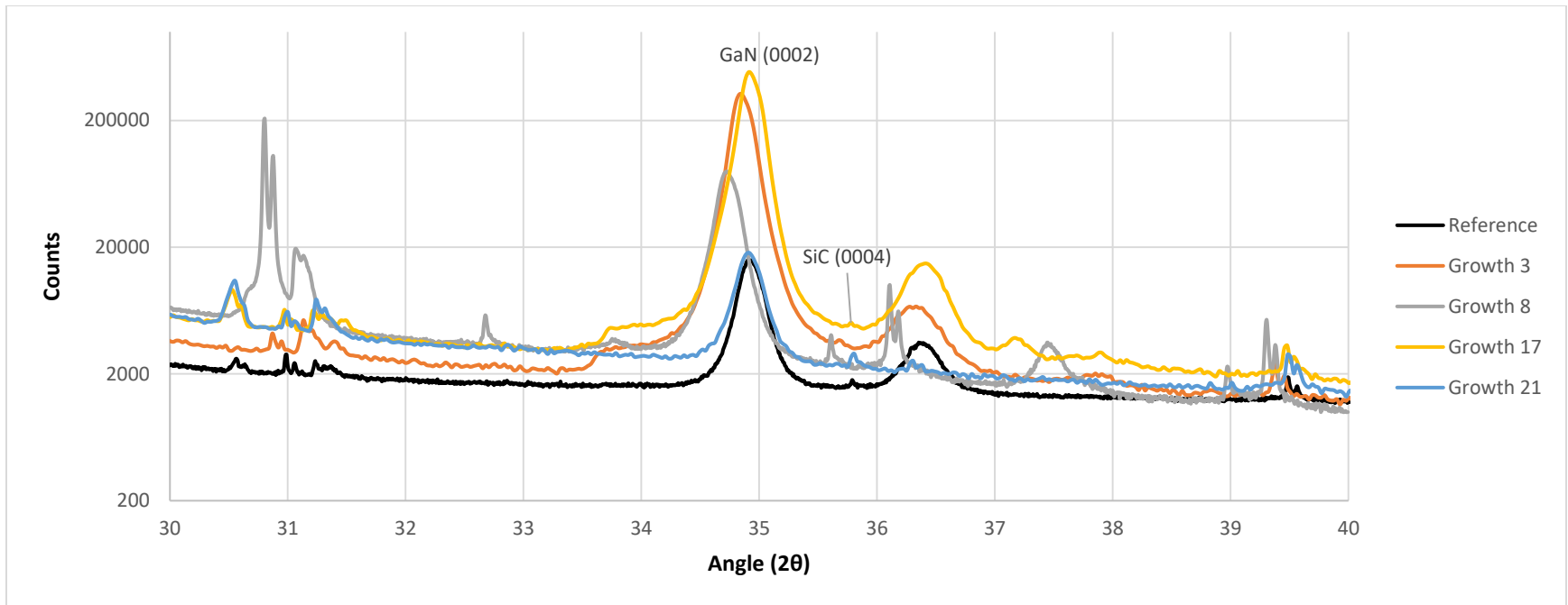
Figure 26 AlN XRD Plots
