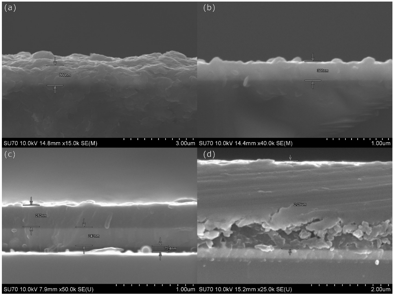
Figure 20 SEM images with thickness measurements for (a) Growth 3, (b) Growth 8, (c) Growth 17 and (d) Growth 21
