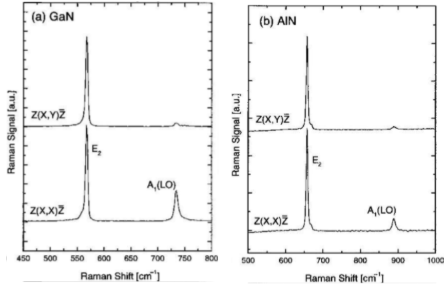
Figure 11 Raman spectra for (a) GaN and (b) AlN at room temperature. [34]
