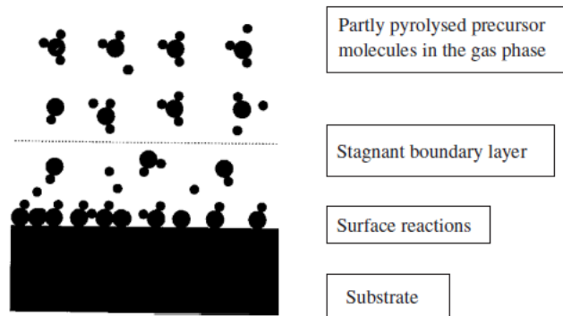
Figure 13 Simple schematic representation of the MOCVD process. [37]
