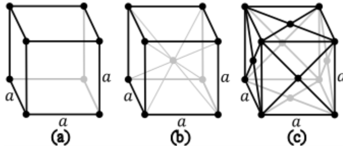
Figure 3 The three varieties of cubic systems (a) primitive, (b) body centered (c) face centered
