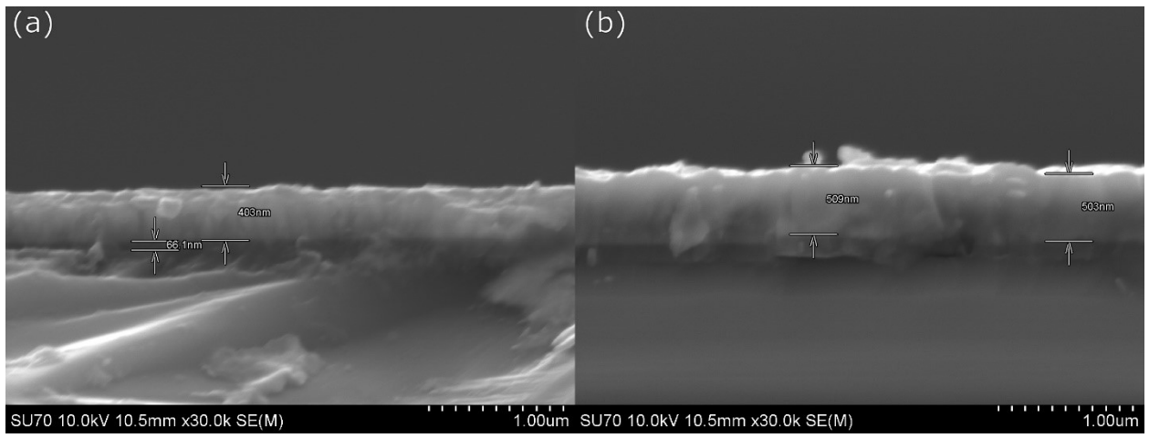
Figure 29 SEM results for GaN (a) growth 10 (b) growth 19.
