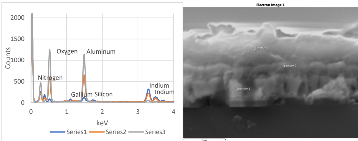
Figure 36 EDX and corresponding SEM image for growth 16.
