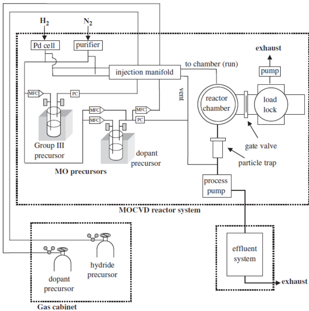
Figure 14 Schematic diagram of a MOCVD reactor. [37]
