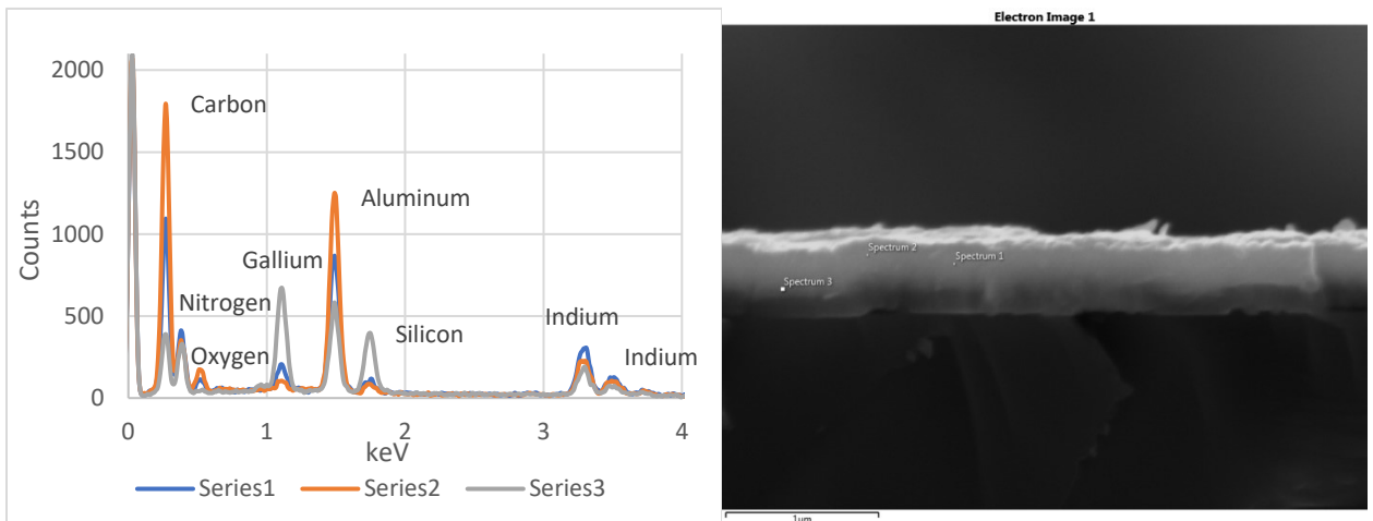
Figure 35 EDX and corresponding SEM image for growth 11.
