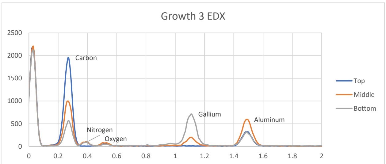
Figure 21 EDX graph for growth 3
