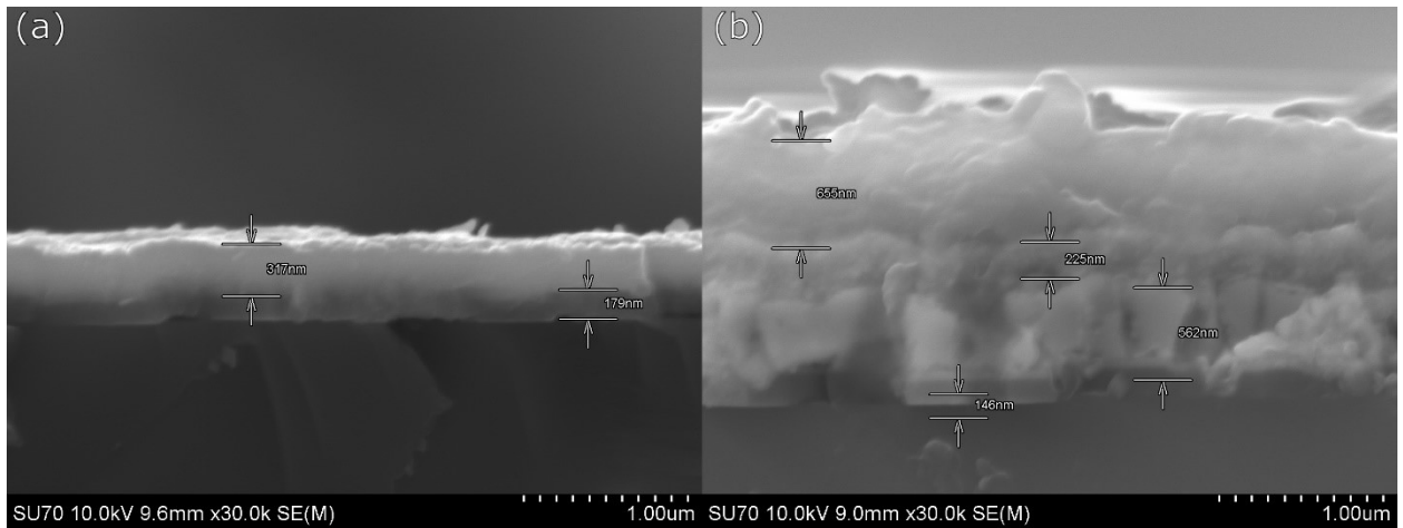
Figure 34 SEM images for InAlN for (a) growth 11 and (b) growth 16.
