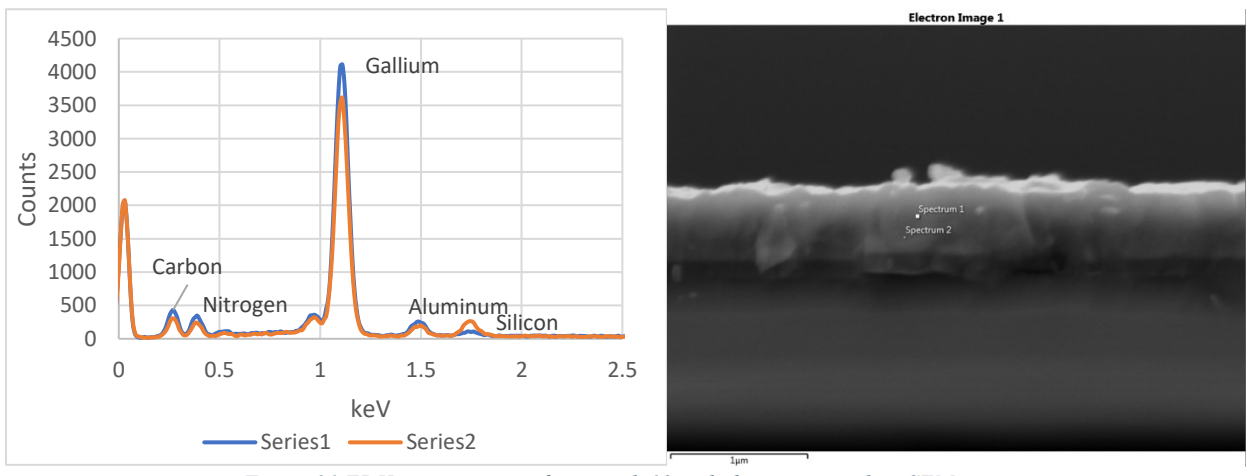
Figure 31 EDX measurements for growth 19 with the corresponding SEM image
