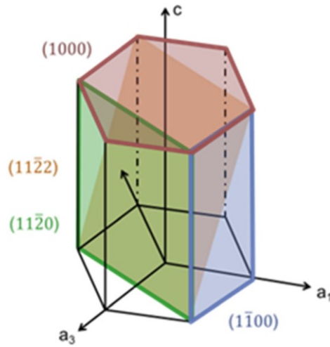
Figure 2 Basic wurtzite crystal showing axis and common planes [6]
