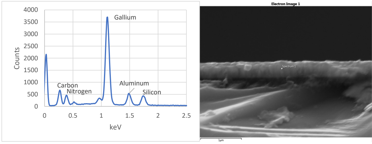
Figure 30 EDX measurement for growth 10 with the corresponding SEM image
