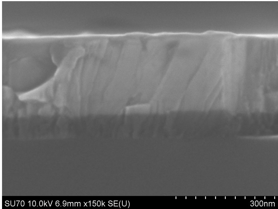
Figure 17 SEM image of the SiC Template The light grey area is the GaN and the dark great area is SiC, under the SiC is silicon
