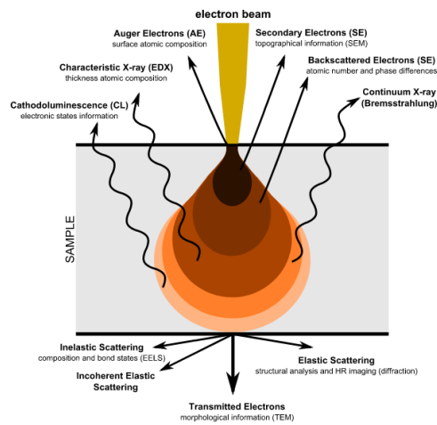
Figure 9 Interaction bloom in a sample caused by the interacting electrons. [32]
