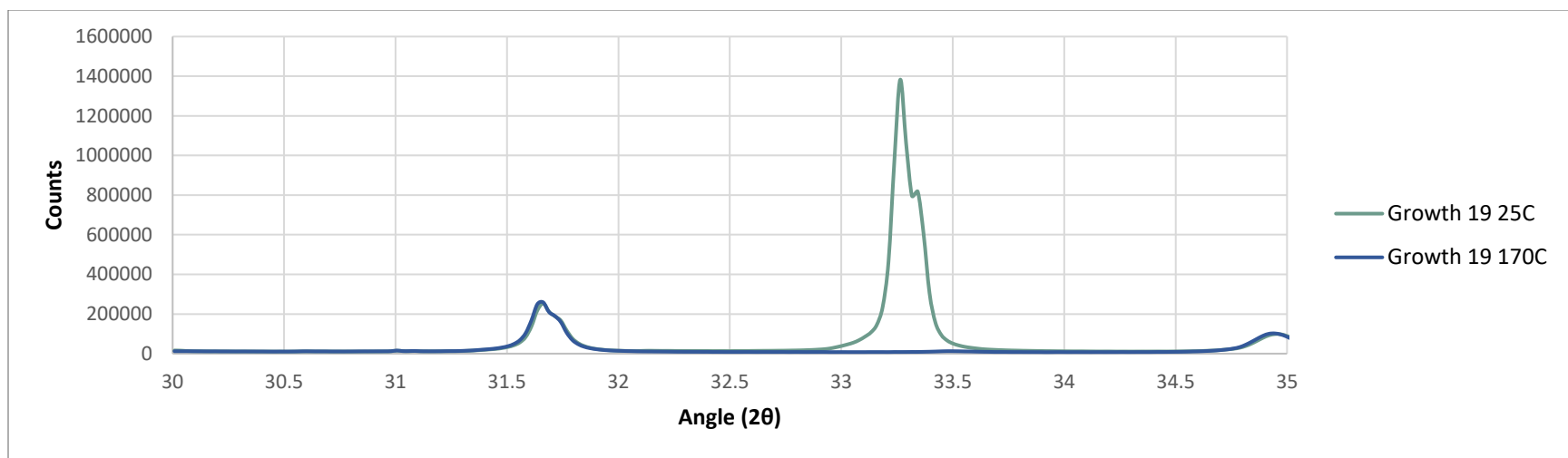
Figure 39 XRD scan of growth 19 at room temperature and at 170°C
