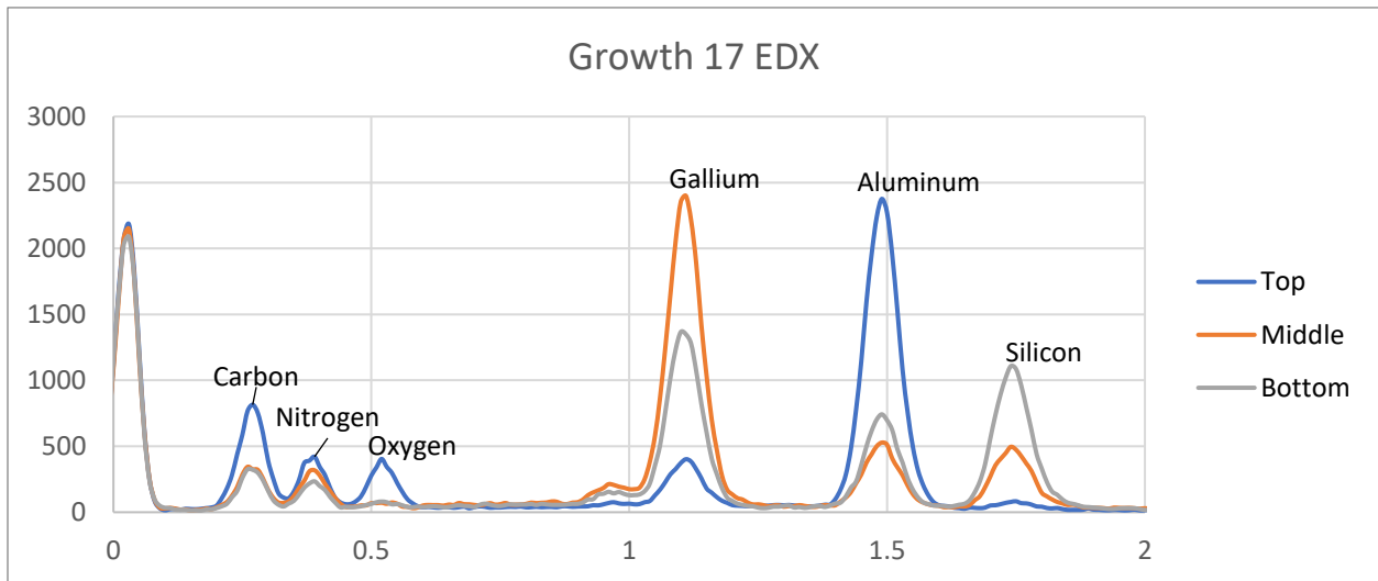
Figure 23 EDX graph for growth 17
