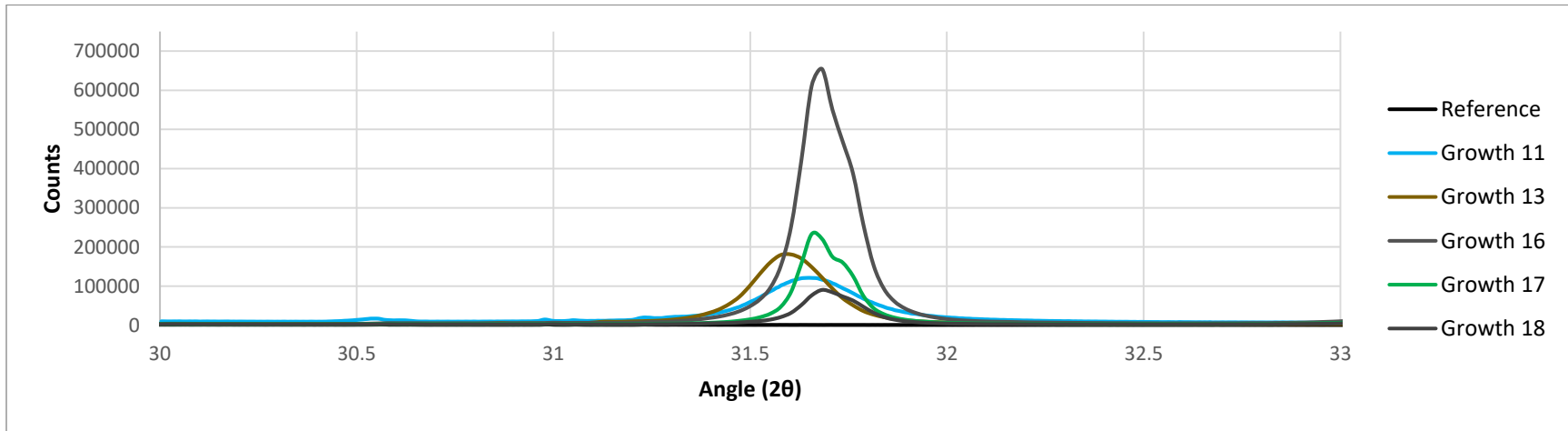
Figure 38 XRD scans on InAlN
