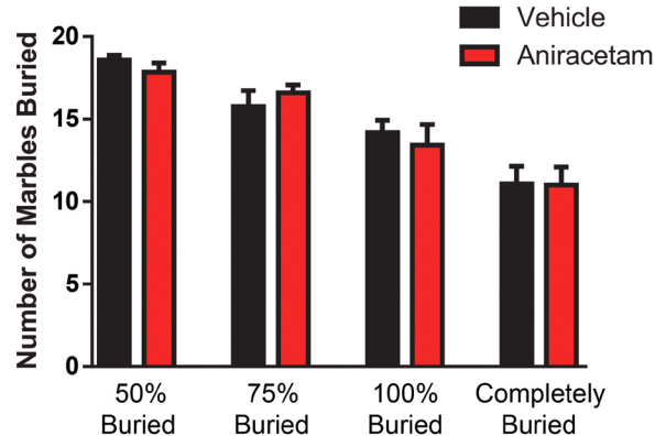
Figure 3. Aniracetam pretreatment does not change performance on the marble burying task. Independent measures t-tests revealed no significant differences in the animal's performance in marble burying when measured at: 50% t(1,22) = 1.18 , p = 0.24 ; 75% t(1,22) = 0.76 , p = 0.45 ; 100% t(1,22) = 0.50 , p = 0.61 ; or at the level of completely buried t(1,22) = 0.05 , p = 0.95 .
