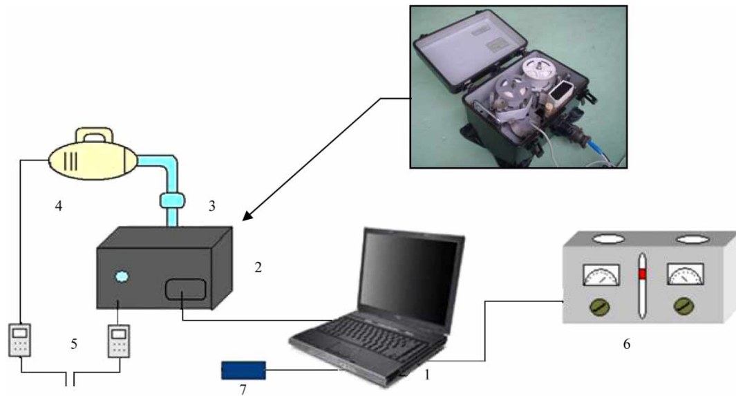
Fig. 2. Measurement scheme: 1 – computer; 2 – filtration device; 3 – air volume meter; 4 – air pump; 5 – stopwatches; 6 – optical aerosol particle counter; 7– multifunctional data logger
