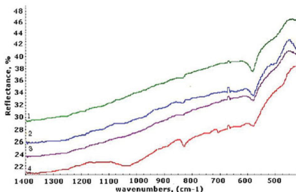
Fig. 6. Results of FTIR spectroscopy investigation of corrosion products on the zinc-polymeric coatings under different environment conditions: 1 – reference (not exposed); 2 – marine; 3 – rural-agrarian; 4 – industrial
