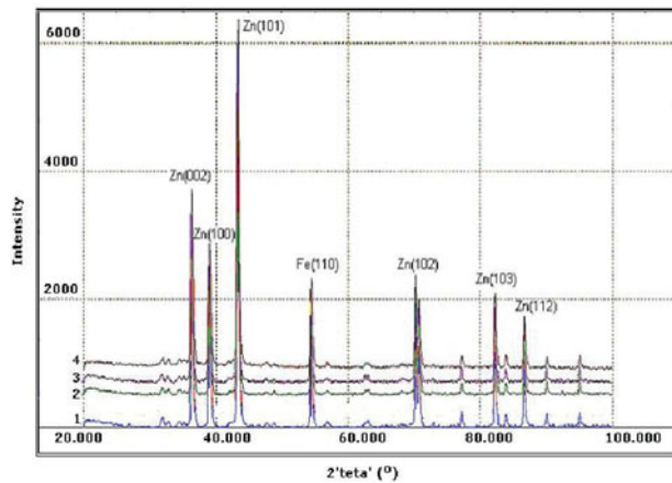
Fig. 7. Phase composition of coatings determined by XRD method under different environment conditions: 1 – reference (not exposed); 2 – marine; 3 – rural-agrarian; 4 – industrial
