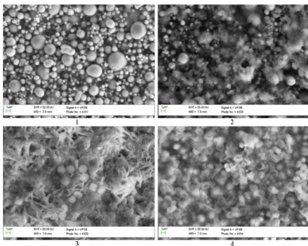
Fig. 4. The changes in the surfaces of zinc-polymeric coatings on steel after 1.5 years of exposure to different environment conditions: 1 – reference (not exposed); 2 – marine; 3 – rural-agrarian; 4 – industrial
