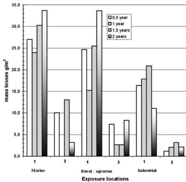
Fig. 8. Mass losses (1) after removal of corrosion products and mass change (2) after exposure of zinc-polymeric coatings versus the duration of exposure
