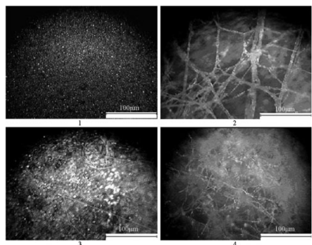
Fig. 3. Micrographs of zinc-polymeric coatings on steel under different environment conditions: 1 – reference (not exposed); 2 – marine; 3 – rural-agrarian; 4 – industrial
