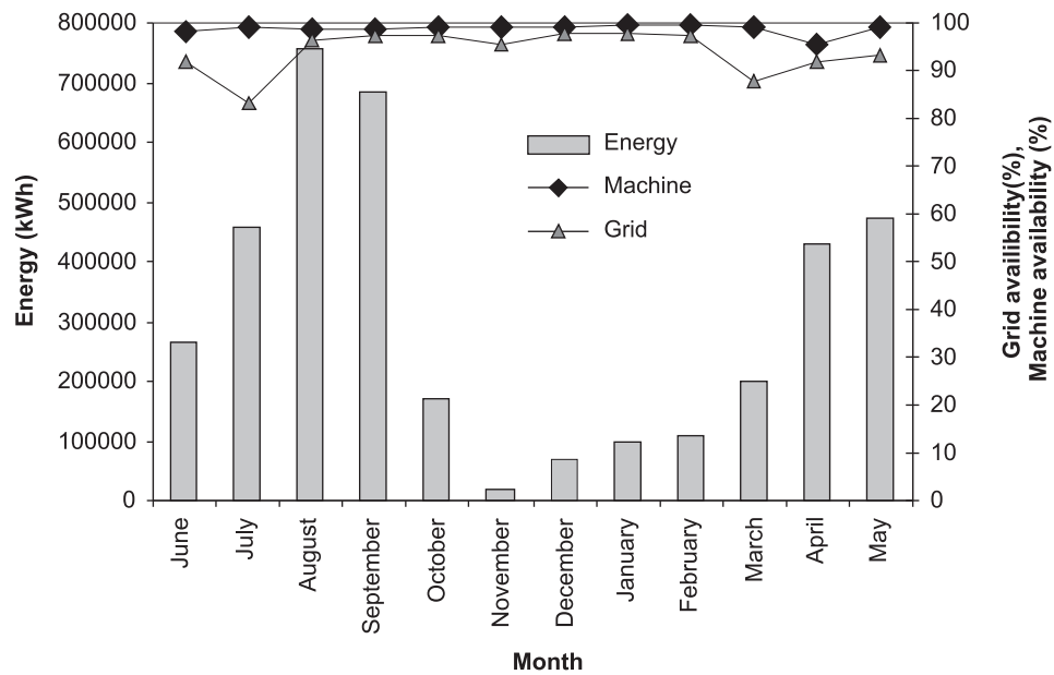
Figure 1: Annual energy generation, machine availability, and grid availability of the Motha site
