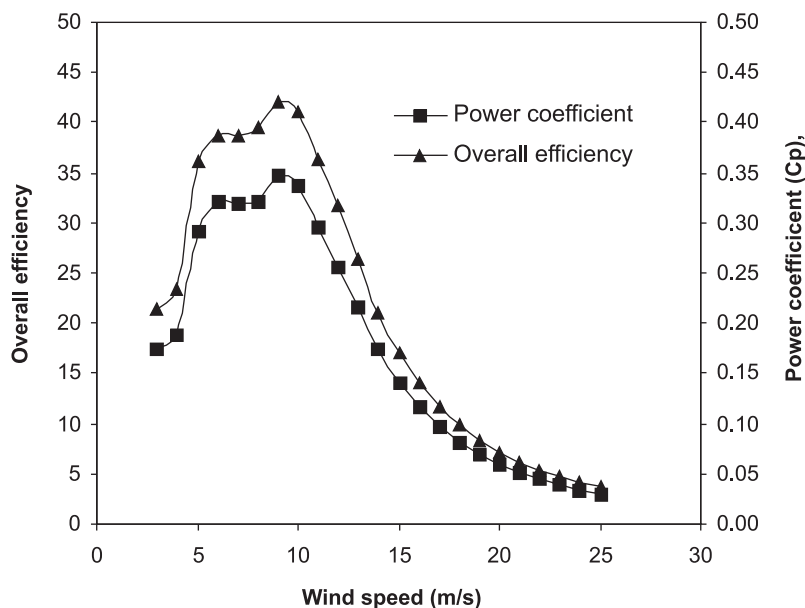
Figure 4: Power coefficient and overall efficiency of 1 MW capacity wind turbine
