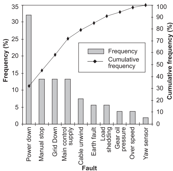
Figure 3: Fault analysis by using the Pareto Chart for the wind farm, Motha
