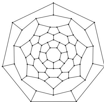
Fig. 3. The basic graph for the set S_{3,4,9,85+}
