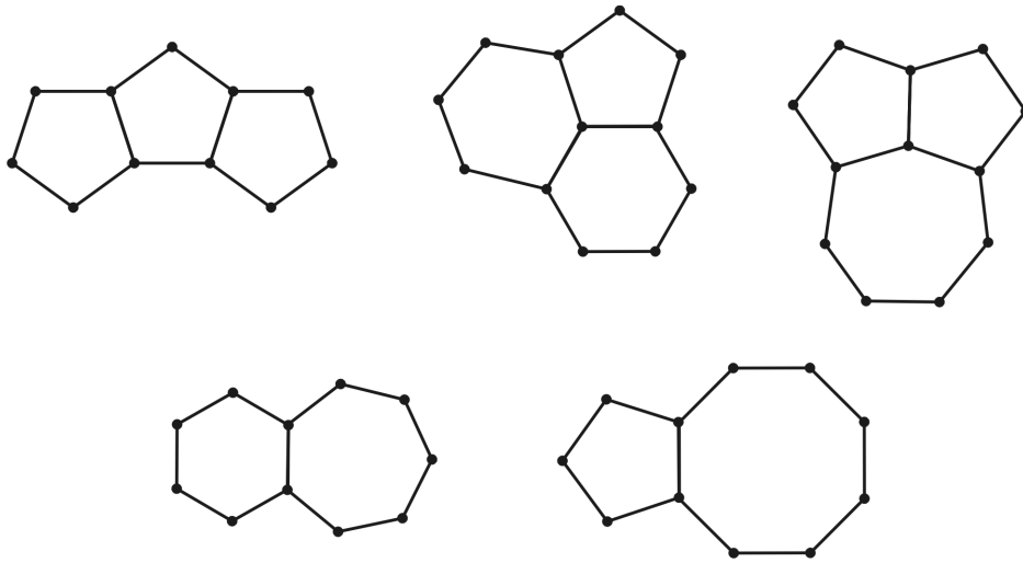
Fig. 7. Five forbidden clusters of faces
