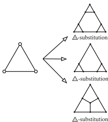
Fig. 2. The \triangle -, \triangle - and \triangle -substitutions
