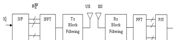
Fig. 1 UFMC System Model
