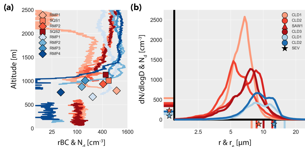
Figure 4. Cloud microphysical properties and rBC for the 31 August (red) and 4 September (blue) flights. (a) Vertical profiles of rBC number concentration (lines) and average N_d (markers) for each RMP and SQS profile. The vertical positions of the markers indicate cloud-top height for each profile and the horizontal positions indicate the average N_d value. Note that rBC and N_d share the same x axis because they have the same units and similar magnitudes. (b) Average cloud droplet spectra (curves), N_d (ticks on y axis), and r_e (ticks on x axis) for each CLD and SAW leg. Stars indicate the values of N_d and r_e from SEVIRI (SEV) averaged over the 31 August (light red) and 4 September (light blue) flight paths.
