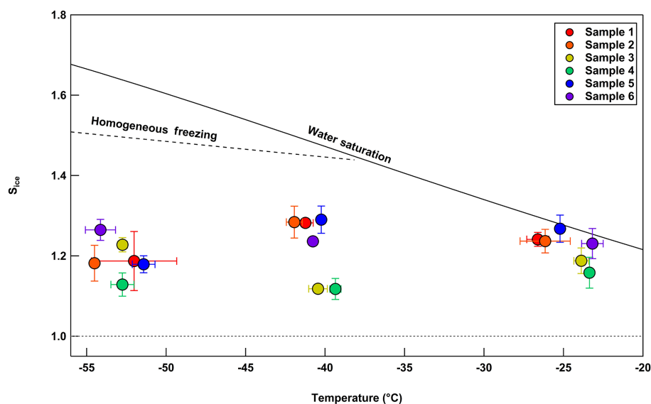
Figure 10. Depositional ice nucleation experiments on samples 1–6 plotted by S_{ice} versus temperature. The values plotted here are of the onset conditions of depositional ice nucleation. For our experiments, this refers to the first particle to nucleate ice out of the 10^4 particles deposited on the disc in total, thus a percent activated fraction of 10^{-4} . Although temperatures measured were not exactly -25 , -40 , and -55 °C, these values are used for brevity for all samples within each grouping shown above. Nucleation occurring at -25 °C could also be due to immersion freezing.
