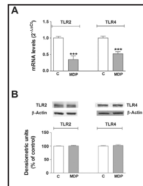
Fig. 5. NOD2 modulates TLR2 and TLR4 expression. Cells were treated with MDP 50 \mu\text{g/ml} for 1 day. A. Real-time PCR analysis of TLR2 and TLR4 mRNA expression in treated cells. Relative quantification was performed using comparative Ct method ( 2^{-\Delta\Delta\text{Ct}} ). Results are expressed as arbitrary units (control = 1) and are the mean \pm SEM of four independent experiments. B. Immunodetection and quantification of TLR2 and TLR4 protein expression in cell lysate using \beta -actin as an internal control of the protein load (TLR2 and TLR4/ \beta actin ratio). The results are expressed as a percentage of the control value (100%) and are the mean \pm SEM of five independent experiments. *** P < 0.001 compared with the control value.
