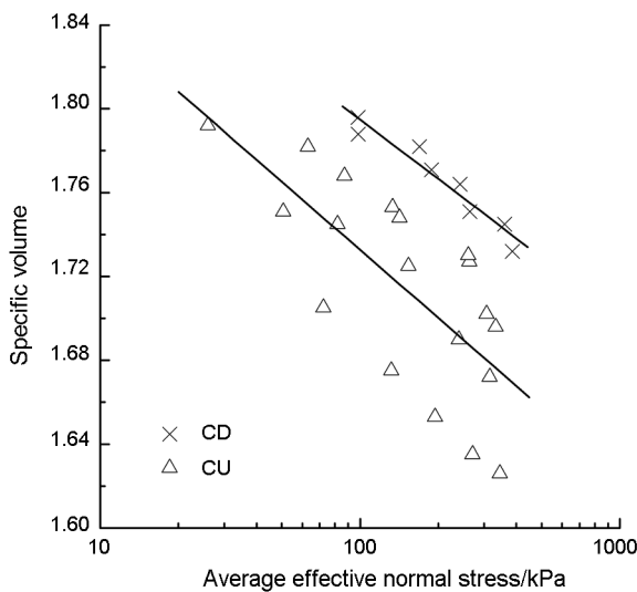
Fig. 3. Comparison between p' and v under different drainage conditions
