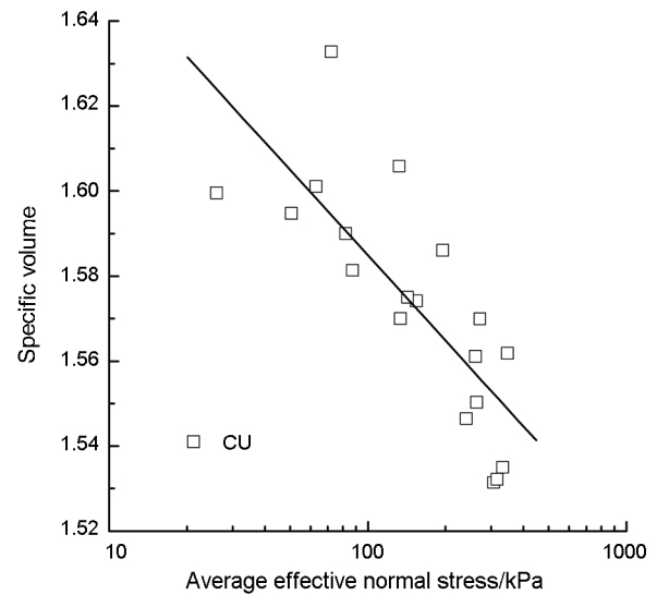
Fig. 4. Relationship between p' and v after normalization
