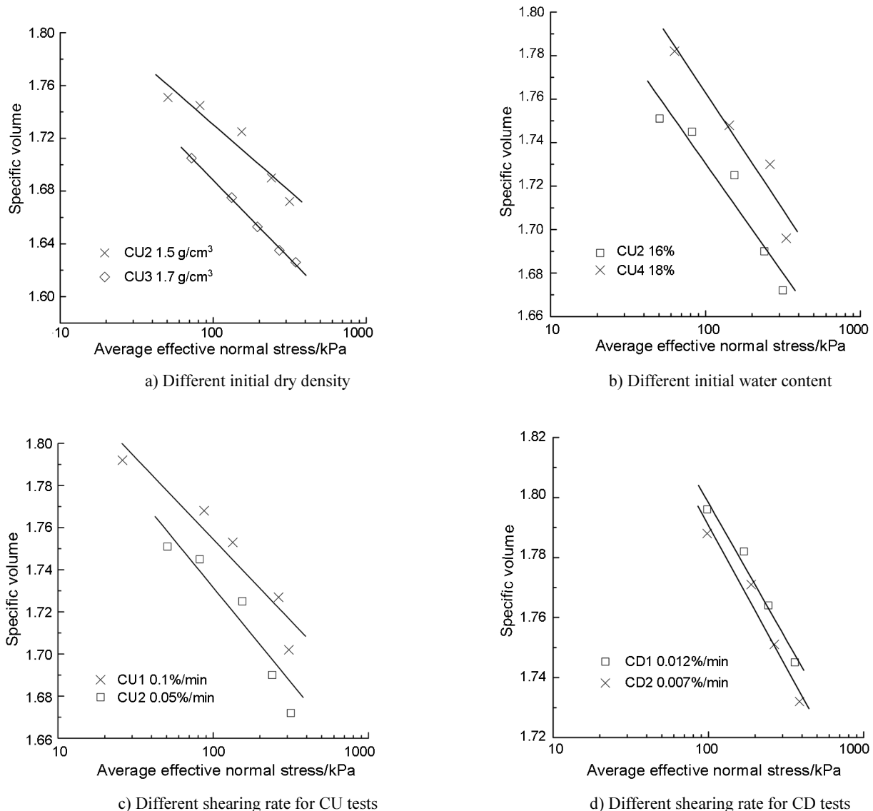
Fig. 2. Relationship between average effective normal stress and specific volume under different parameters
