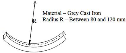
Figure 3: Ring specimen
