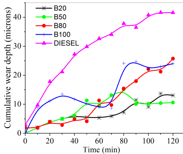
Figure 7: Comparison of wear depth between the various blends.
