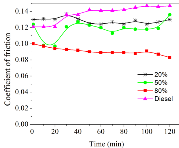
Figure 6: Comparison of coefficient of friction between various blends obtained from a reciprocating wear test.
