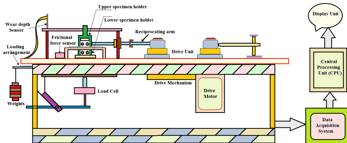
Figure 2: Schematic sketch of the reciprocating friction and wear testing machine.
