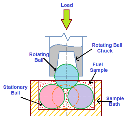
Figure 1: Four ball tester.
