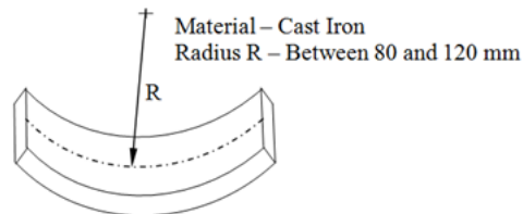
Figure 4: Liner specimen.
