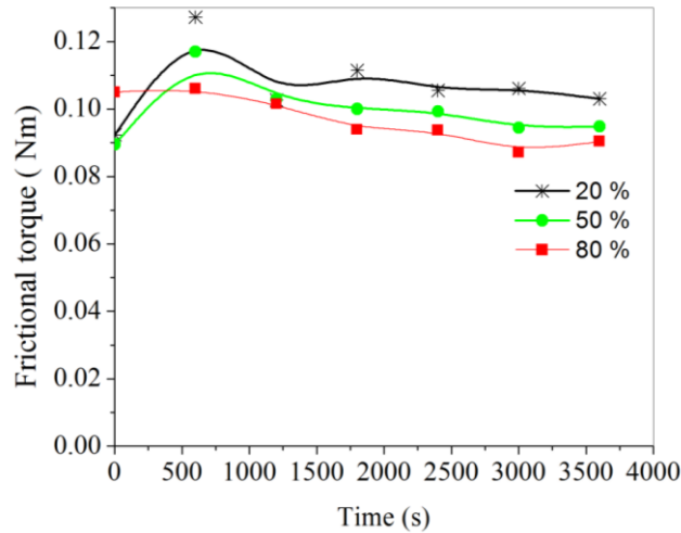
Figure 5: Comparison of frictional torques between samples tested with various blends in a four ball tester.
