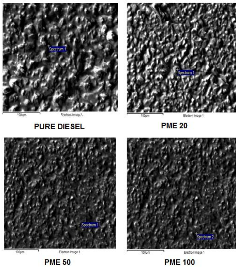
Figure 9: SEM images of worn cylinder surfaces for different lubricating oils.
