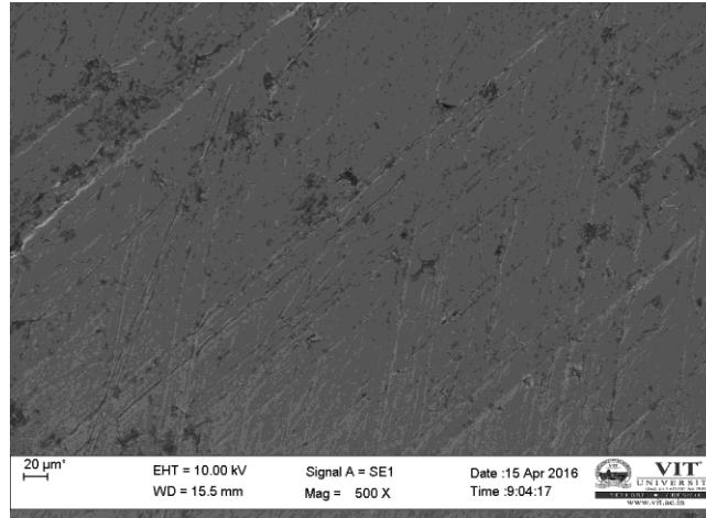
Figure 8: SEM image of the liner at a less wear affected zone.
