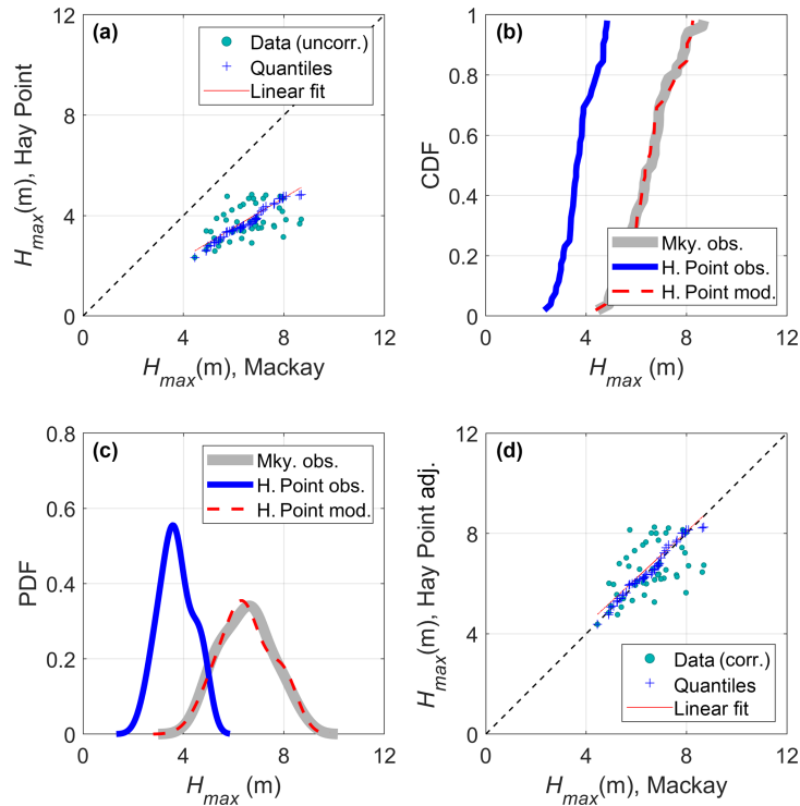
Figure 2. Example of the CDF mapping approach used to extrapolate an estimate of H_{\max} at the Mackay wave buoy, using data from the Hay Point buoy. (a) shows the raw observations (green) and quantiles (blue) of H_{\max} at both sites during the overlapping period; (b) shows the cumulative distribution of H_{\max} at Hay Point (observed, blue line), at Mackay (observed, grey line), and at Hay Point (CDF mapped to Mackay, red dotted line); (c) shows the same for the probability density of H_{\max} , and (d) shows the CDF-adjusted Hay Point data against the original Mackay data, demonstrating their improvement as a predictor for H_{\max} at Mackay, compared to (a).
