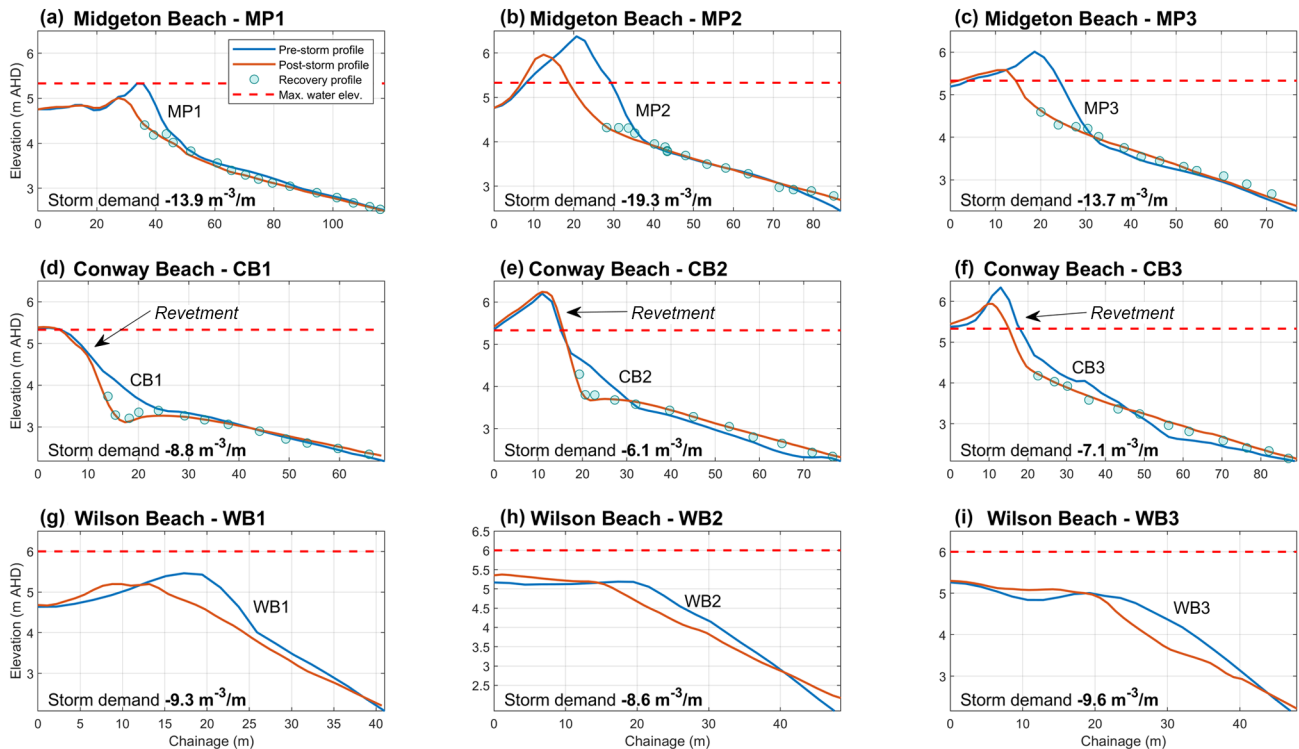
Figure 8. Cross-shore beach profile change at Midgeton Beach (a–c), Conway Beach (d–f) and Wilson Beach (g–i). Blue (orange) lines denote pre- (post-) storm profiles taken through the lidar DEMs (locations Fig. 9). Green circles show alongshore-averaged DGPS elevations along the same profile lines \sim 5 months after Debbie . Only the lower “recovery” profile is shown at Midgeton Beach because heavy vegetation hindered DGPS data collection. Only the lower “recovery” profile is shown at Conway Beach because the upper portion is a revetment. No “recovery” profiles are shown for Wilson Beach because beach recharge occurred in the interim. Also shown is the estimate of maximum water elevation from Fig. 6 and storm demand. (f) indicates the revetment has moved during Debbie along profile CB3, consistent with observations (DSITI, 2017). The storm demand calculation for CB3 does not include the revetment change.
