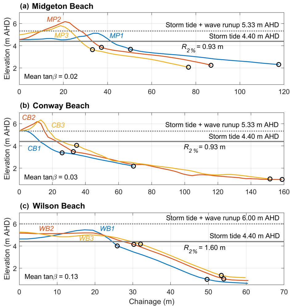
Figure 6. Pre-Debbie beach profiles (July–August 2016) at (a) Midgeton Beach, (b) Conway Beach and (c) Wilson Beach (profile locations in Fig. 7). Maximum storm tide elevation was taken from the nearest gauge (Laguna Quays) (grey solid line), and maximum water elevation (grey dashed line) was defined as R_{2\%} + storm tide elevation. R_{2\%} corresponds to the expected level of exceedance of 2% of the wave runups during wave conditions at the time of maximum storm tide elevation ( H_{s0} 5 m L_0 131 m, at 12:00 28 March). R_{2\%} was calculated for each location based on the mean slope ( \tan \beta ) of the profiles. The locations at which \tan \beta was calculated for each profile are shown (base of dune to toe of upper beach, black circles).
