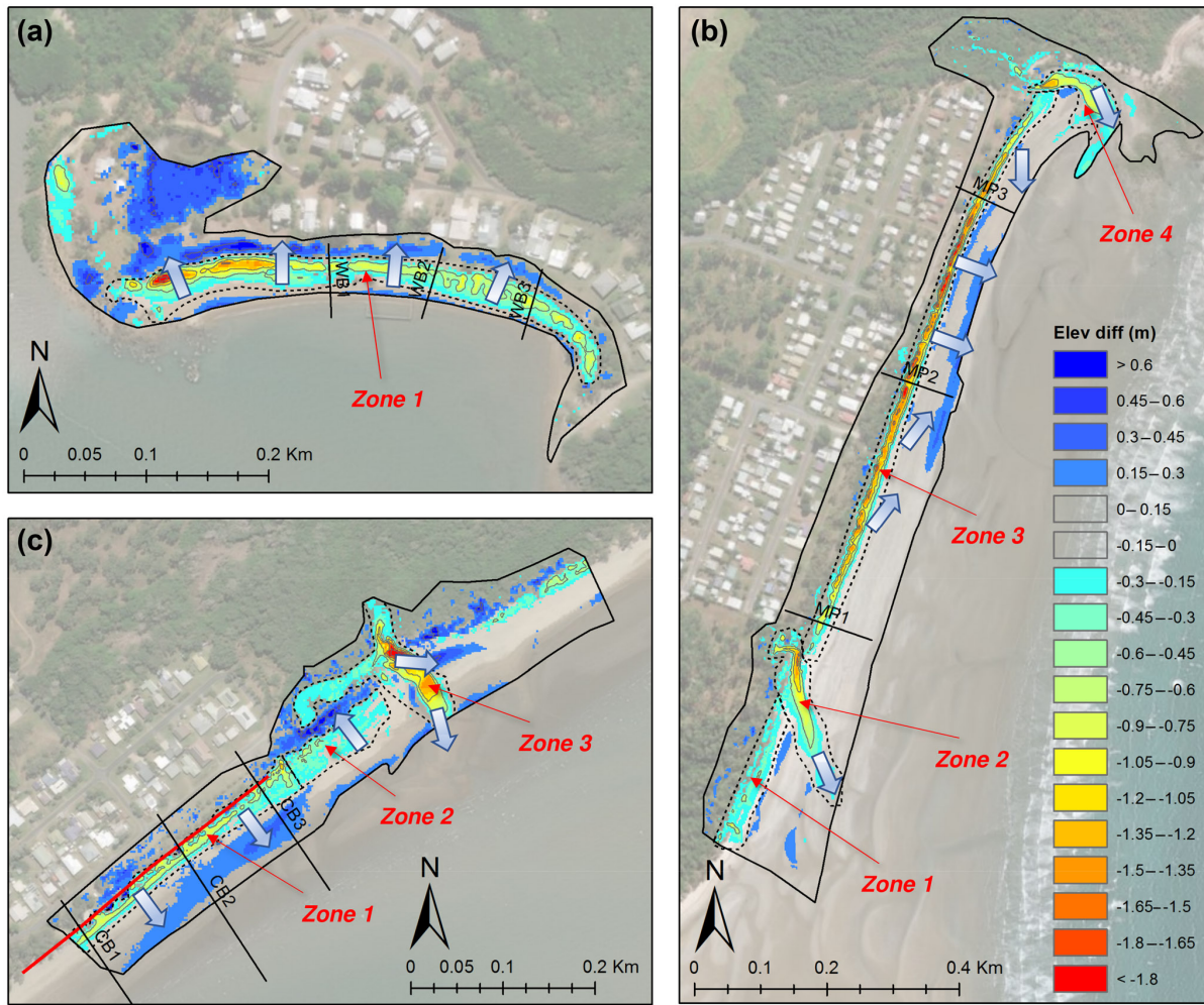
Figure 7. Coastal erosion, deposition and inferred transport pathways during Debbie at (a) Wilson Beach, (b) Conway Beach and (c) Midgeton Beach. Elevation difference plots show changes in metres (pre- Debbie minus post- Debbie ), with \pm 0.15 m (reported vertical error of lidar) not shown. Contours at 1.5, 1.0, 0.5, -0.5 , -1 , -1.5 and -2.0 are overlaid (grey lines). The approximate position of the rock revetment at Conway Beach is shown in (b) (red line). Also shown are locations of cross-shore beach profiles at each site, extents of Fugro Roames lidar data used (black box), and erosion zones referred to in the text (dashed lines).
