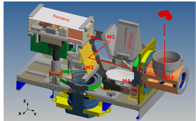
Figure 2. WIRA-C optics with flat mirror M3 (inside the scan-drum), flat mirror M2 (on a linear stage), elliptical mirror M1, elliptical mirror M4 (sleuable, drawn in inactive state), hot load and the front end with the feed horn.
