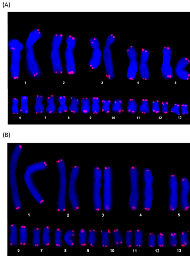
Fig. 4. Fluorescence in situ hybridization (FISH) with telomeric probe exclusively mapped (TTAGGG) n repeats to terminal regions of all chromosomes of K. eiffingeri (a) and K. idiootocus (b). No interstitial telomeric sequence (ITS) was detected in both species.
