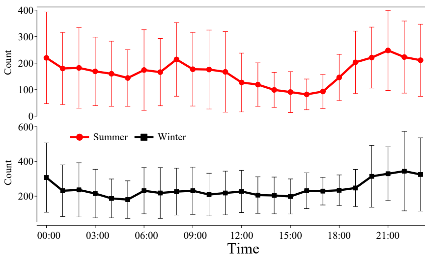
Figure 3. Diurnal variations in amine-containing particle counts in summer and winter in Heshan.
