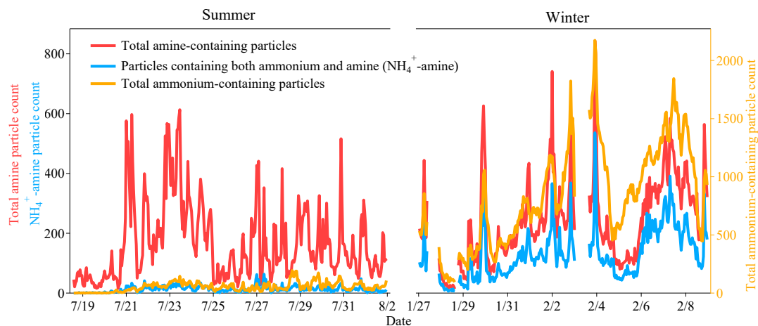
Figure 7. Temporal variations in total amine-containing particles, total ammonium-containing particles, and particles containing both ammonium and amine ( \text{NH}_4^+ -amine) during sampling period in Heshan.
