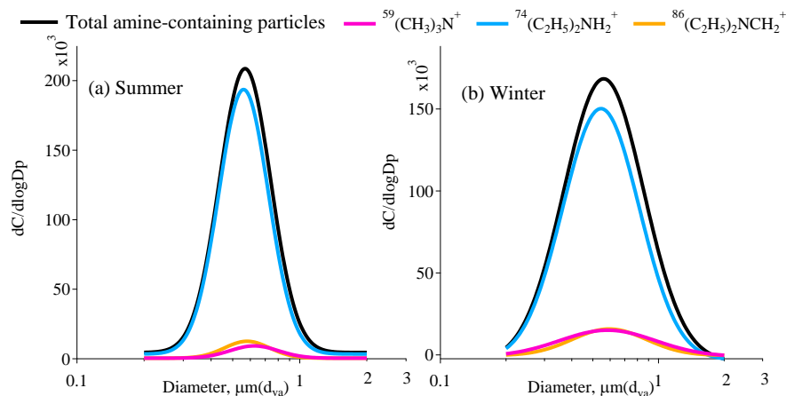
Figure 5. Unscaled size-resolved number distributions of total amine-containing particles and amine particles containing the three marker ions of ^{59}(\text{CH}_3)_3\text{N}^+ , ^{74}(\text{C}_2\text{H}_5)_2\text{NH}_2^+ , and ^{86}(\text{C}_2\text{H}_5)_2\text{NCH}_2^+ in summer and winter in Heshan.
