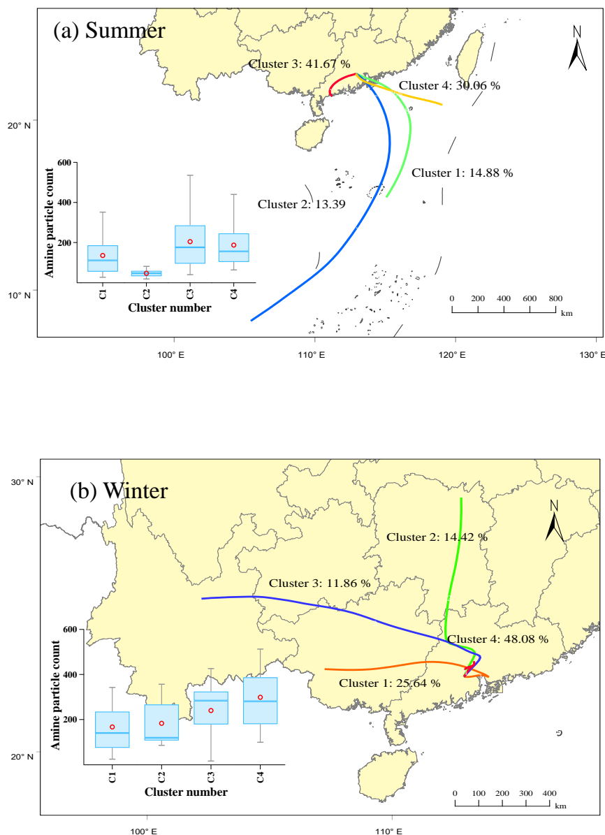
Figure 1. Spatial distributions of amine-containing particle counts associated with backward trajectories (48 h) of air masses at 500 m levels above the ground during the sampling period: (a) summer (from 18 July to 1 August 2014), (b) winter (from 27 January to 8 February 2015).
