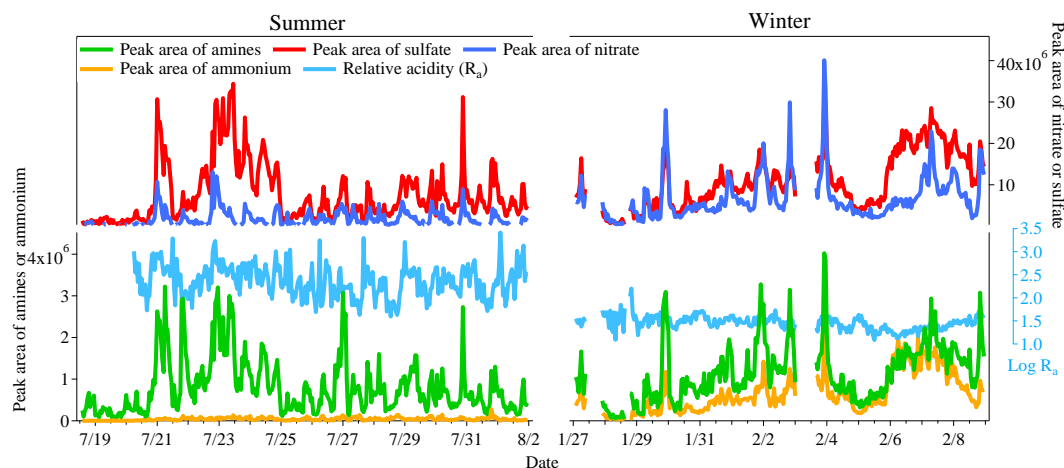
Figure 8. Temporal variations in the peak areas of amines, ammonium, sulfate, and nitrate in amine-containing particles during summer and winter. The relative acidity ratio ( R_a ), which was calculated as the ratio of the total sulfate and nitrate peak areas to the ammonium peak area, is plotted as \log(R_a) .
