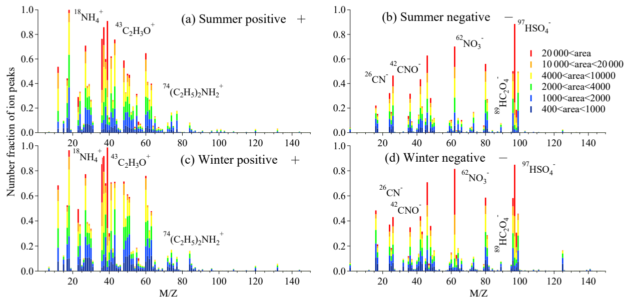
Figure 6. Mass spectra of total ammonium-containing (containing \text{NH}_4^+ ) particles in summer and winter. The color bars represent each peak area corresponding to a specific fraction in individual particles.
