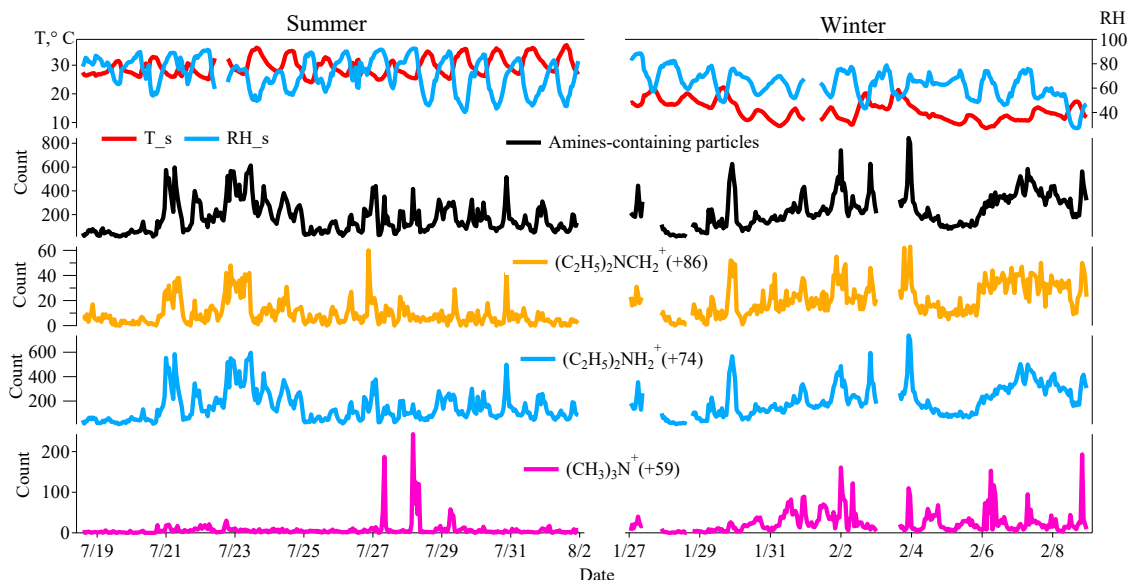
Figure 2. Temporal variations in relative humidity (RH), temperature ( T ), total amine-containing particles, and three major marker ions-containing amine particles ( ^{59}(\text{CH}_3)_3\text{N}^+ , ^{74}(\text{C}_2\text{H}_5)_2\text{NH}_2^+ , ^{86}(\text{C}_2\text{H}_5)_2\text{NCH}_2^+ ) in Heshan, China during the sampling periods.
