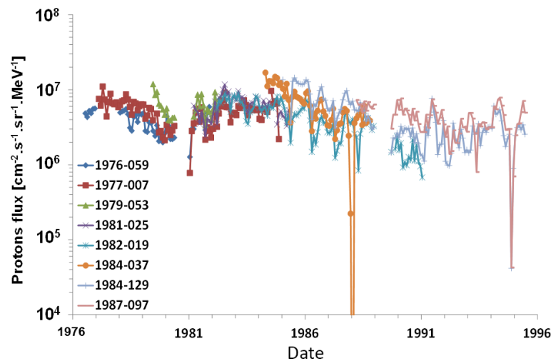
Figure 11. Monthly average 80 keV proton flux measured in GEO by the detector CPA-LoP on board the different LANL satellites.
