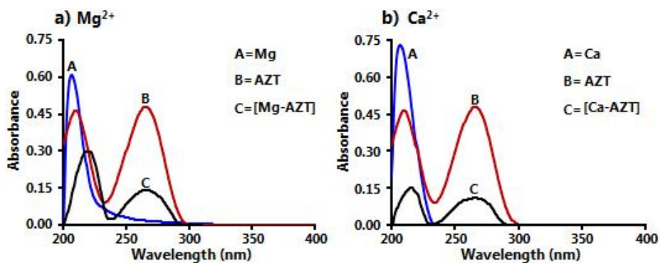
Figure 4. Absorption spectra of (a) Mg^{2+} salt solution, zidovudine and their complex, (b) Ca^{2+} salt solution, zidovudine and their complex in methanol.
