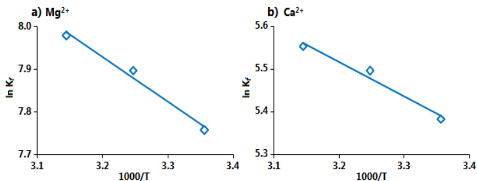
Figure 3. Van't Hoff's plot of \ln K_f vs. 1000/T for the metal complexes with zidovudine (a) Mg^{2+} and (b) Ca^{2+} in methanol.
