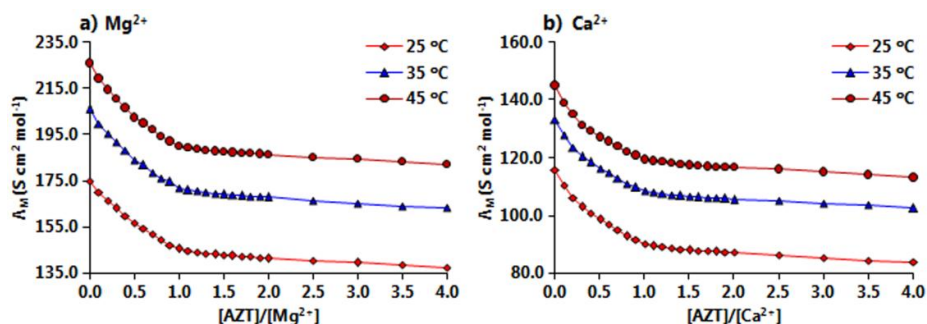
Figure 1. Molar conductance vs. mole ratio [AZT]/[M^{2+}] plots for (a) Mg^{2+} and (b) Ca^{2+} in methanol at 25 °C, 35 °C and 45 °C.
