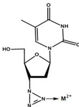
Figure 2. Probable structure of zidovudine-Mg 2+ /Ca 2+ complexes in methanol.
