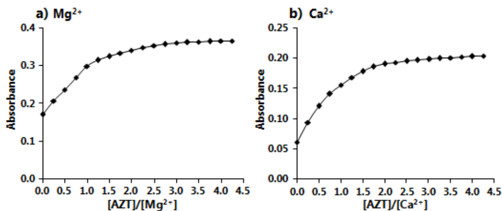
Figure 5. Mole ratio [AZT]/[M^{2+}] plots of (a) Mg^{2+} and (b) Ca^{2+} in methanol at wavelength maxima of 221 nm ( Mg^{2+} -AZT complex) and 216 nm ( Ca^{2+} -AZT complex), respectively.
