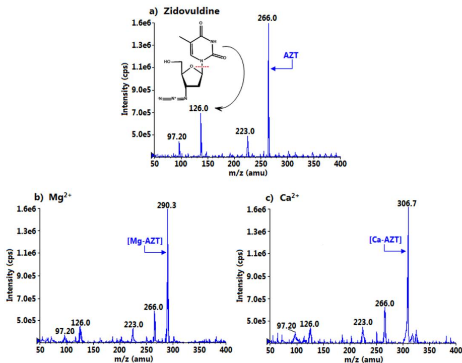
Figure 7. Q1 mass spectra of (a) zidovudine and its complexes with (b) Mg^{2+} and (c) Ca^{2+} cations.
