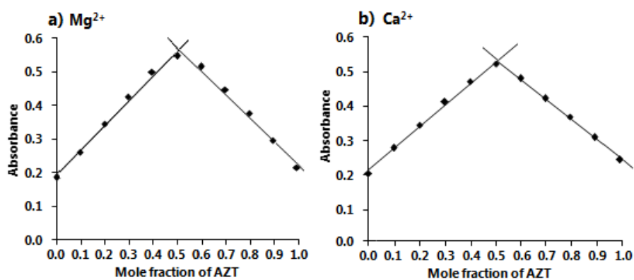
Figure 6. Job's plots for the complexation of zidovudine with (a) Mg^{2+} and (b) Ca^{2+} cations in methanol at wavelength maxima of 221 nm and 216 nm, respectively.
