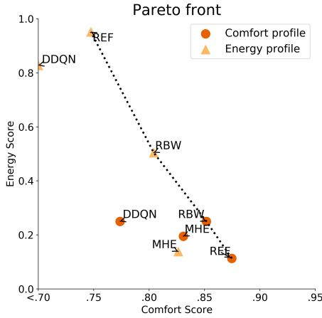
Fig. 6. Performance in occupation profile B
