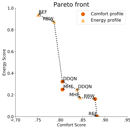
Fig. 7. Performance in occupation profile C
