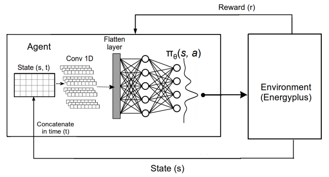
Fig. 4. Reinforcement Learning controller
