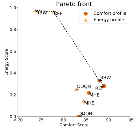
Fig. 5. Performance in occupation profile A
